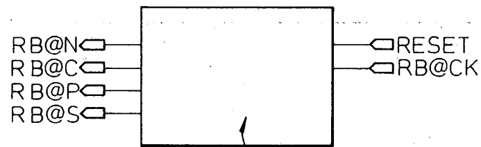
ROW BLOCK STATE LATCH CIRCUIT (HOLDS ONE OF FOUR STATES)
