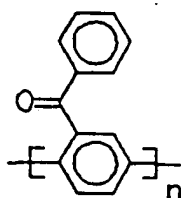
Poly-1,4-(benzoylphenylene), 1
