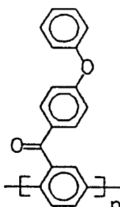
Poly-1,4-(4'-phenoxybenzoylphenylene), 2
