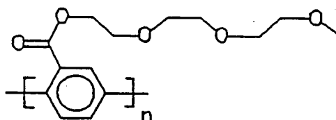
Polymer 3
