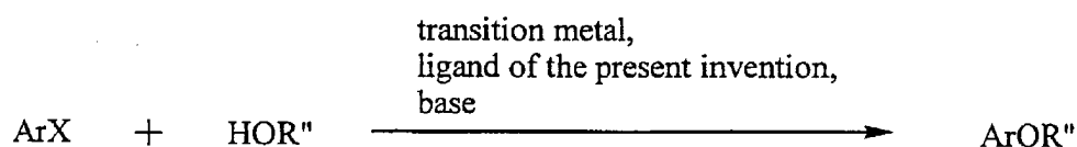
Scheme 6
