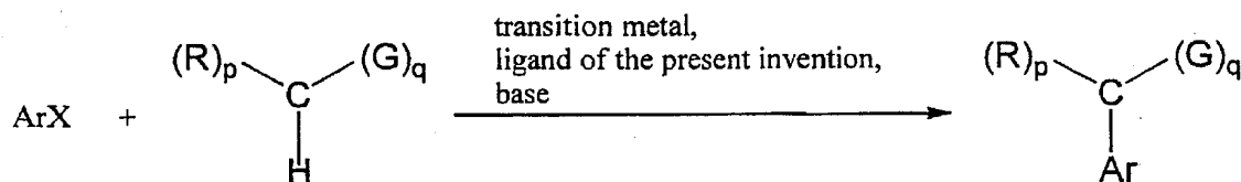
Scheme 4
