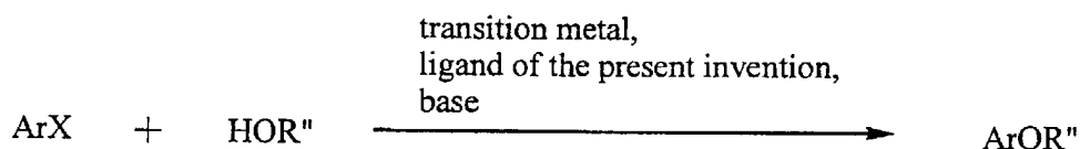
Scheme 6
