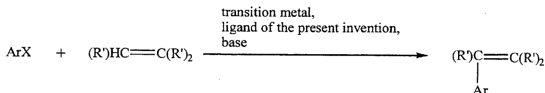
Scheme 8
