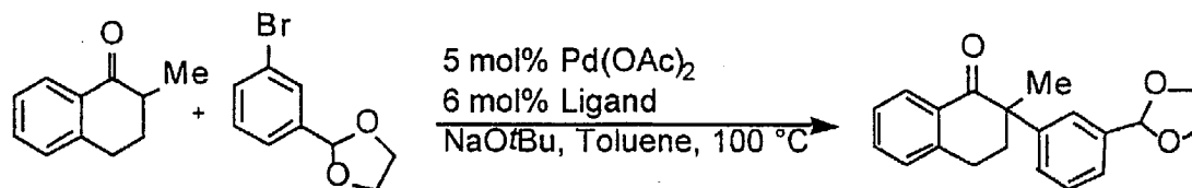
Figure 27 \alpha -Arylation of 2-Methyl-1-Tetralone--Ligand Effects
