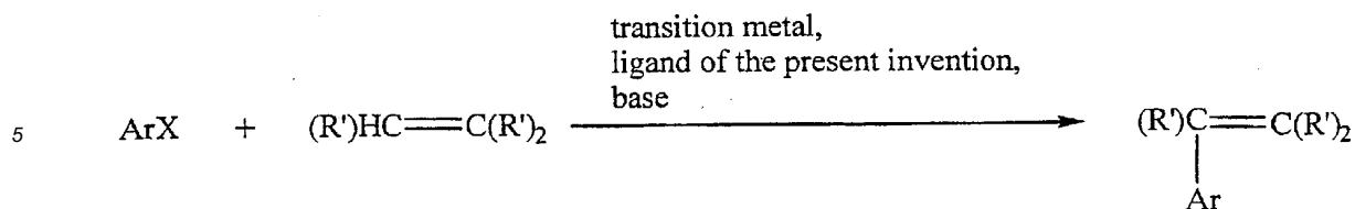
Scheme 8
