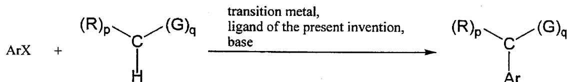
Scheme 4
