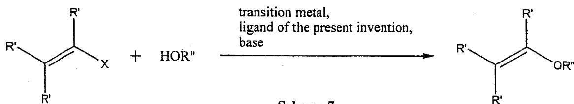
Scheme 7
