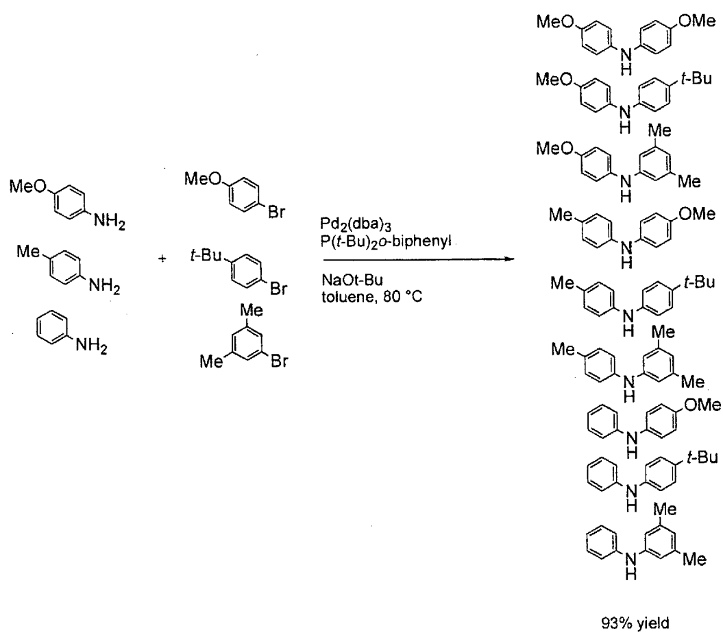
Figure 14 See Example 99.
