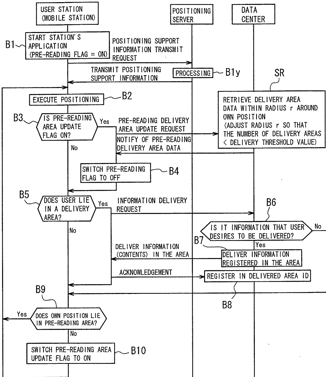
DELIVERY AREA POSITION PRE-READING PROCESS (MEASURING SYSTEM)
