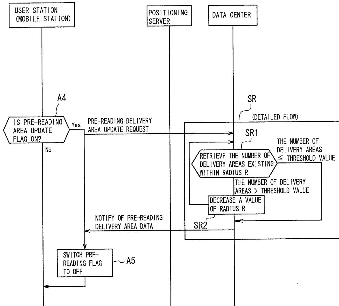
DELIVERY AREA RADIUS ADJUSTING PROCESS
