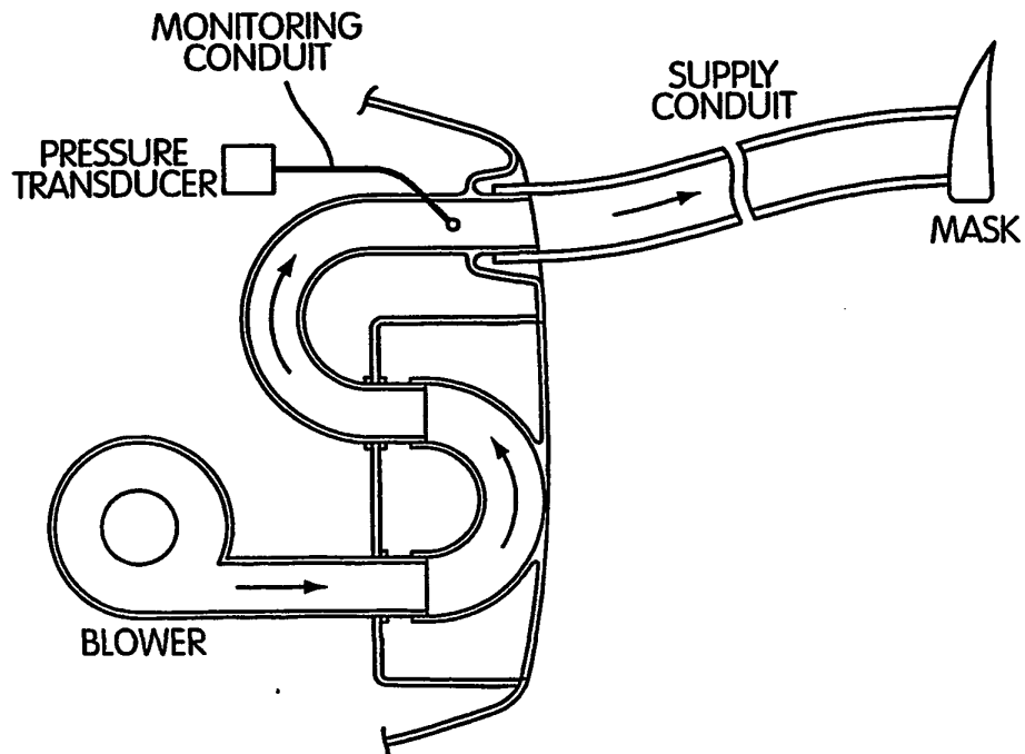
FIG. 29 (RELATED ART)
