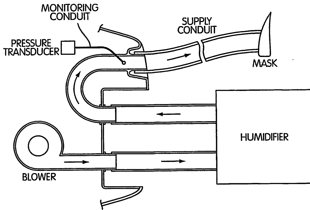
FIG. 28 (RELATED ART)
