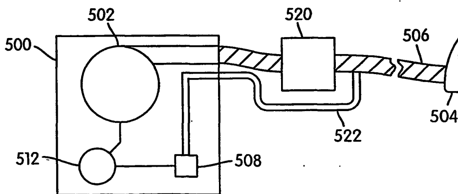
FIG. 27 (PRIOR ART)
