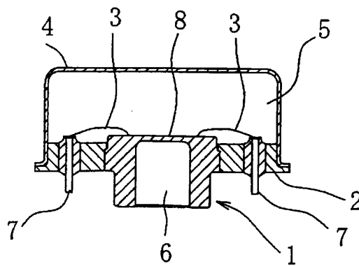
FIG. 11 PRIOR ART
