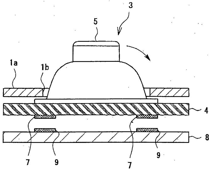
Fig.17A(Prior Art)
