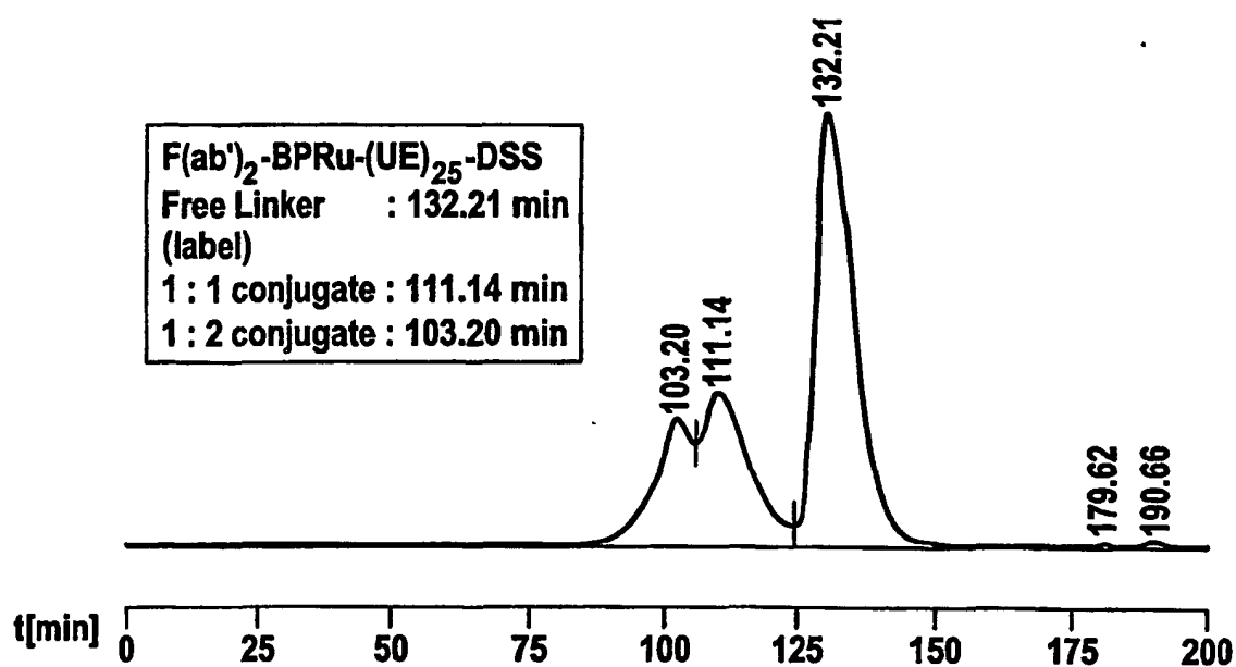
Figure 14: Purification of F(ab') 2 -BPRu-(UE) 25 -DSS coupling products
