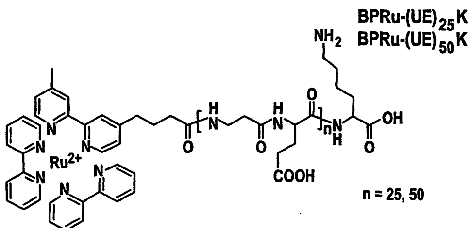
Figure 3: Schematic of BPRu-(UE) 25 K and BPRu-(UE) 50 K
