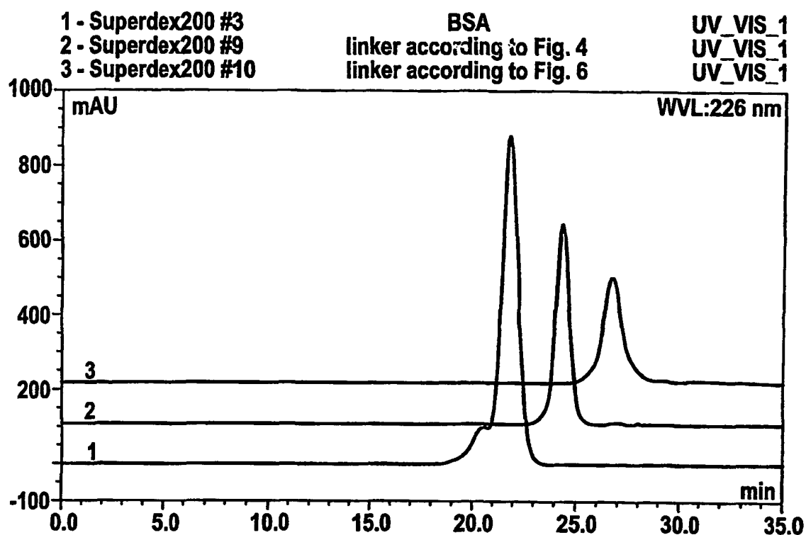
Figure 9: Superdex 200 HR® chromatography of various linker molecules
