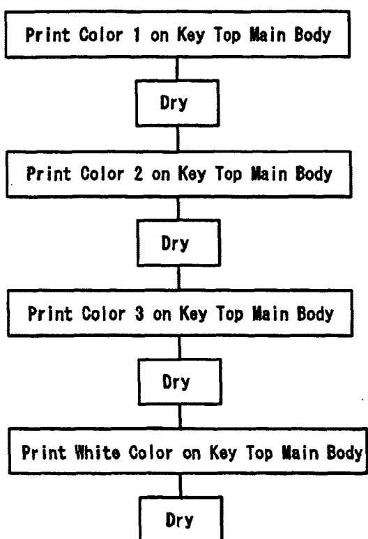
(a) CONVENTIONAL MANUFACTURING FLOW
