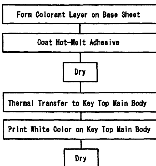
(b) MANUFACTURING FLOW OF PRESENT INVENTION
