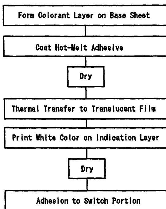
(b) MANUFACTURING FLOW OF PRESENT INVENTION
