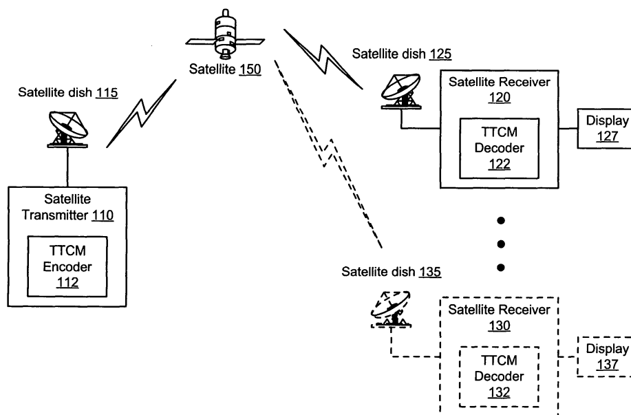
Satellite Communication System 100
