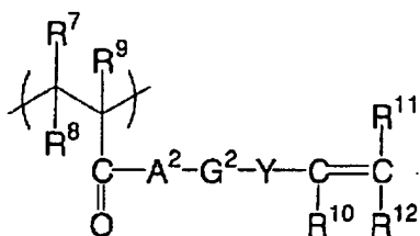
General formula (2)
