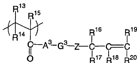
General formula (3)
