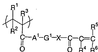
General formula (1)
