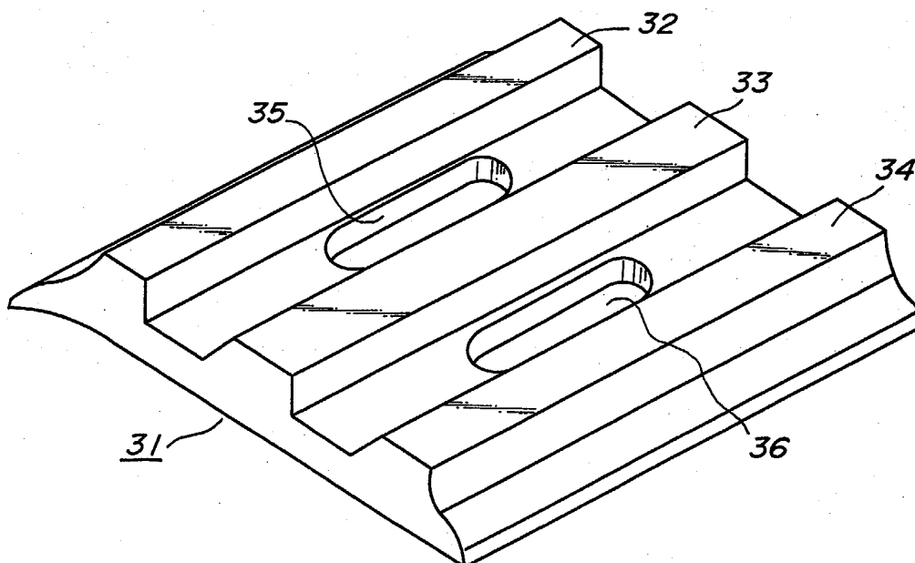
FIG. 17 PRIOR ART
