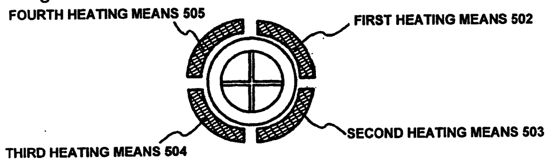
Fig. 5C PLAN VIEW (WHEN DEPOSITION SOURCE IS SET)
