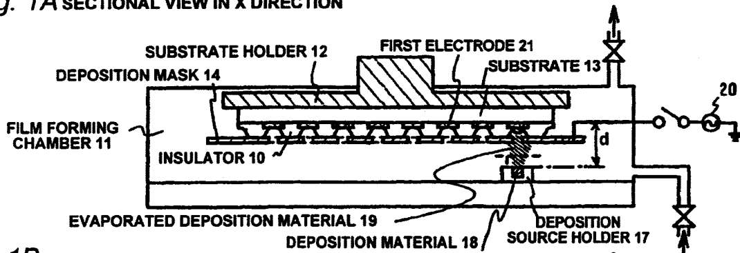
Fig. 1B SECTIONAL VIEW IN Y DIRECTION (IN THE MIDDLE OF FILM FORMATION)
