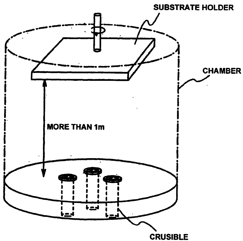
Fig. 11B CONVENTIONAL DEPOSITION APPARATUS
