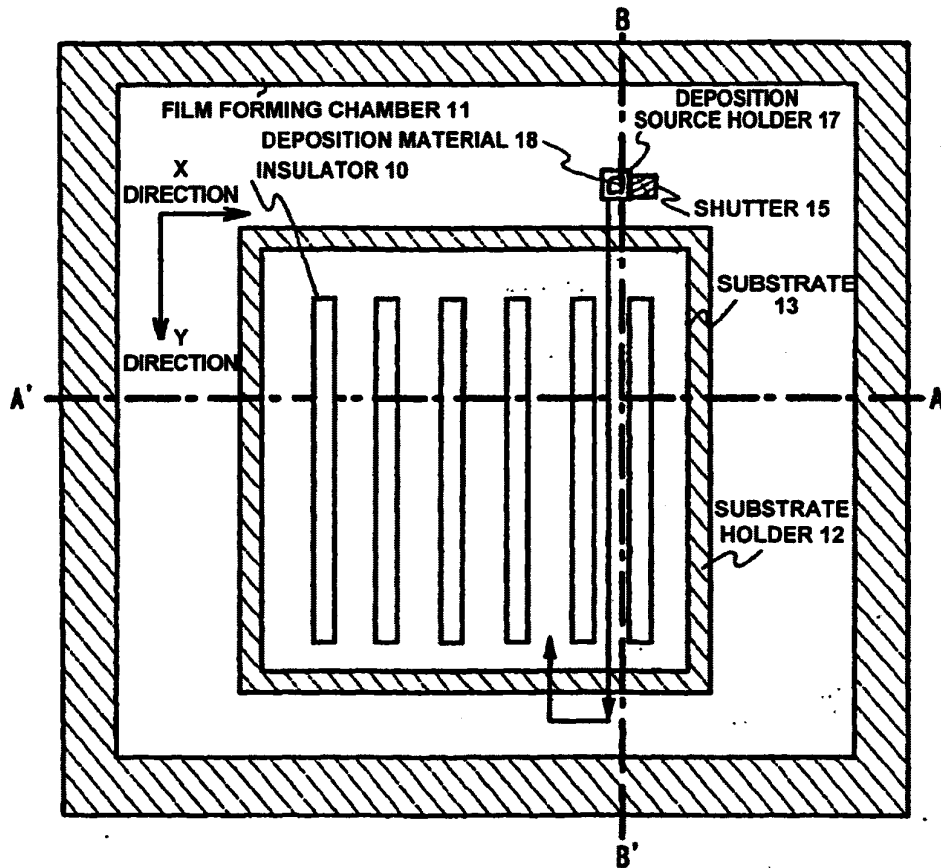
Fig. 1C PLAN VIEW
