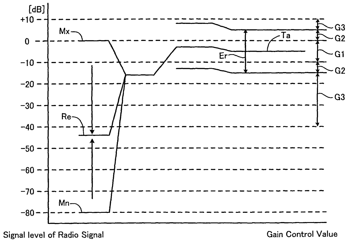
Level Diagram
