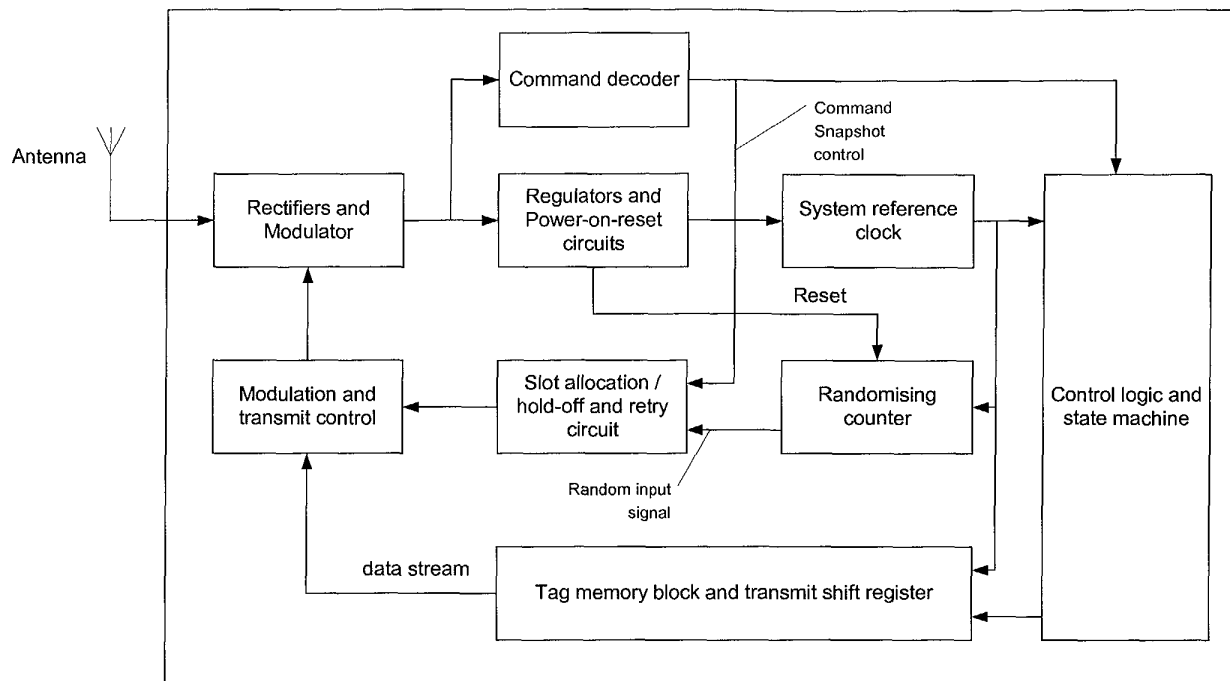
RFID Chip - Block Diagram
