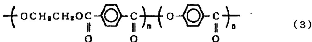
Chemical Formula 3
