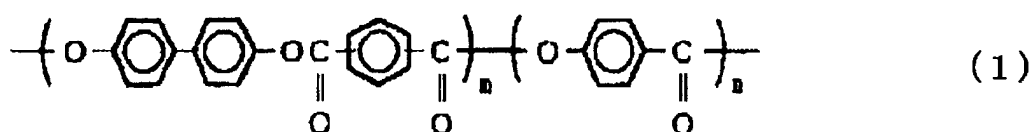
Chemical Formula 1
