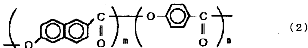
Chemical Formula 2
