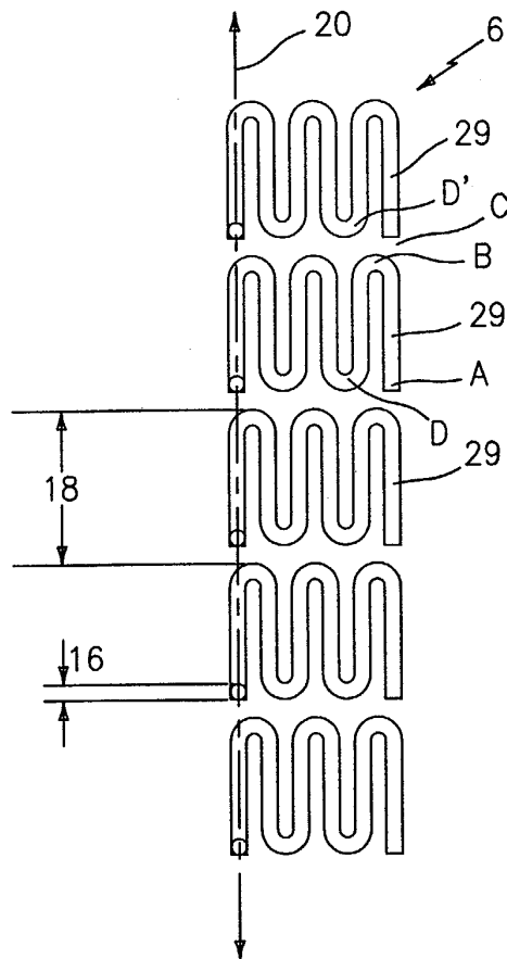
FIG. 4 (PRIOR ART)
