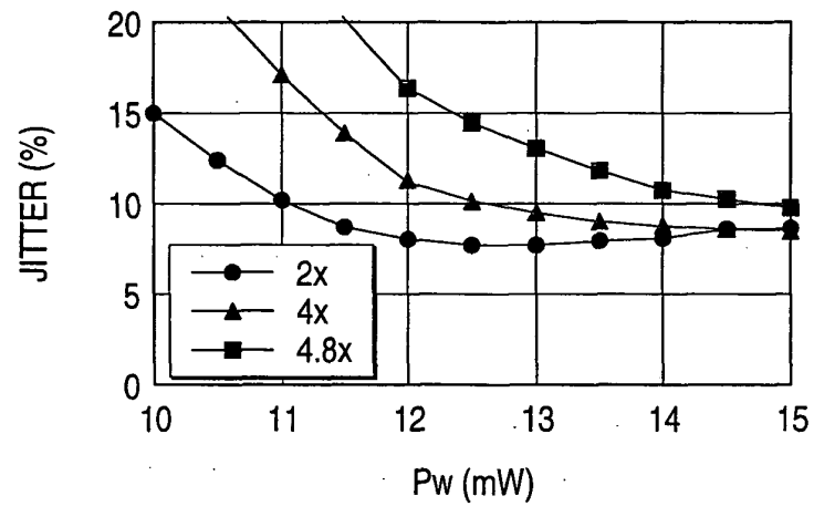
RECORDING POWER DEPENDENCY OF EDGE-TO-CLOCK JITTER
