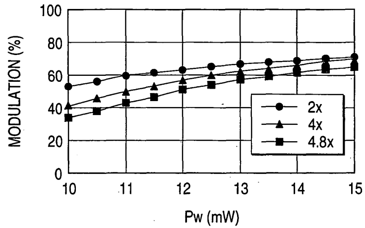
RECORDING POWER DEPENDENCY OF MODULATION
