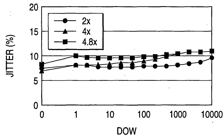
OVERWRITE CYCLE DEPENDENCY OF EDGE-TO-CLOCK JITTER
