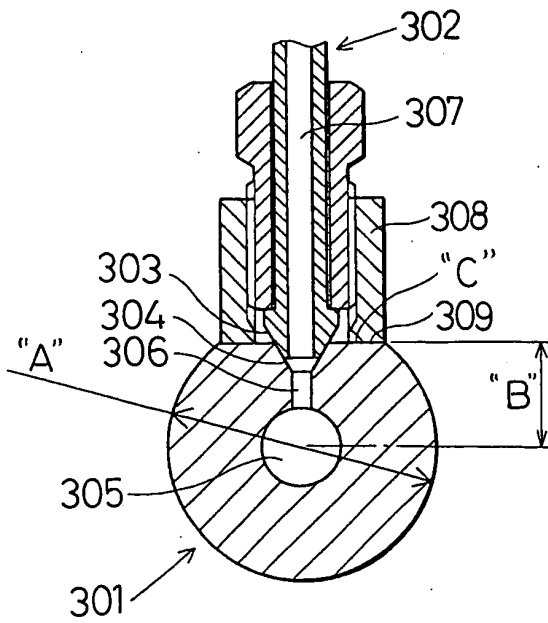
FIG. 14A RELATED ART
