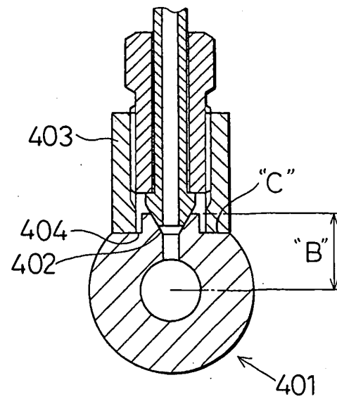
FIG. 14B RELATED ART
