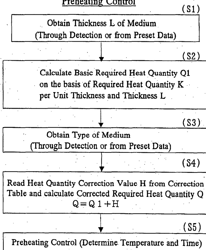
Preheating Control
