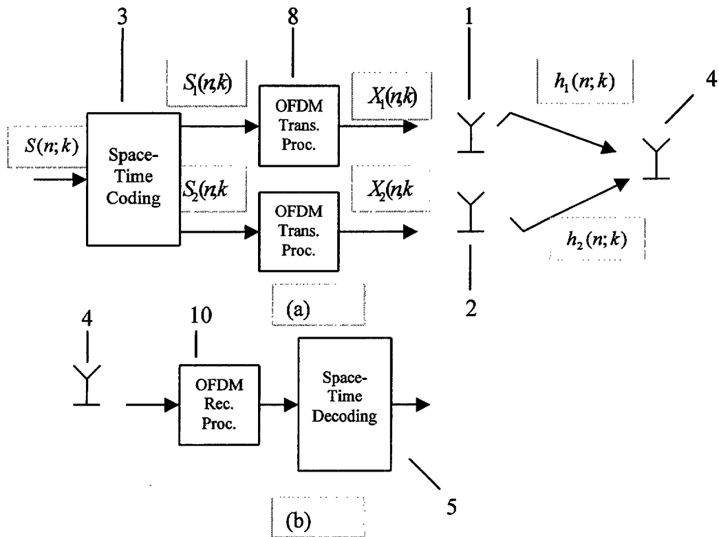
Figure3: Prior Art
