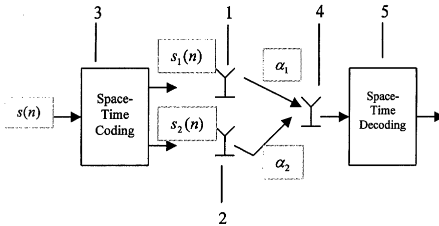
Figure1: Prior Art
