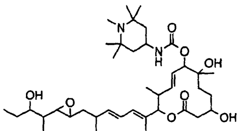
Compound B82
