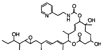
Compound B47
