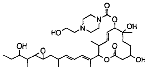
Compound B66
