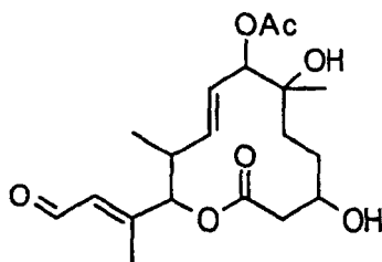
Compound B7
