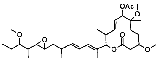
Compound B8-3
