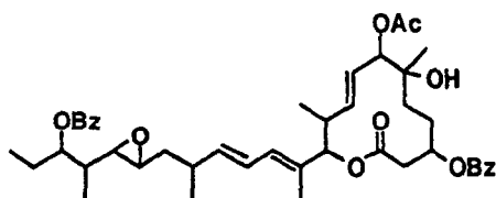
Compound B30-1
