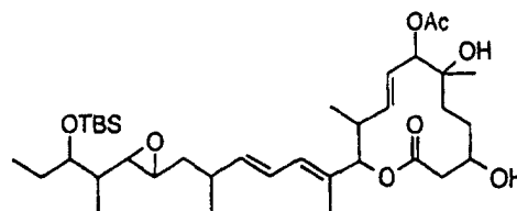
Compound B10-3
