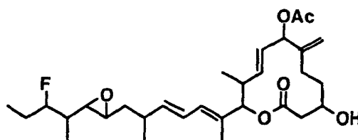
Compound B18-2
