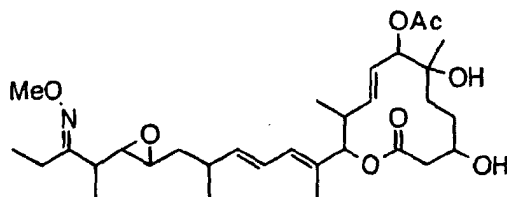
Compound B74
