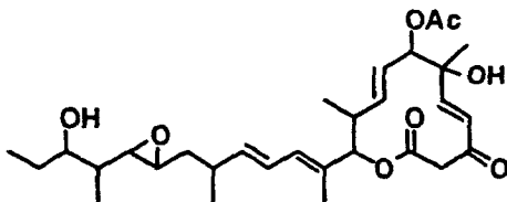
Compound B73
