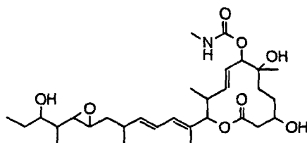
Compound B45
