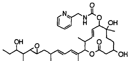
Compound B56
