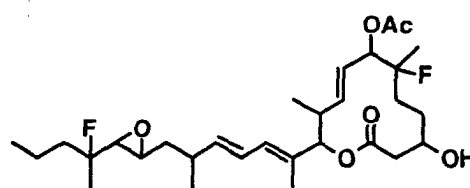
Compound B18-5
