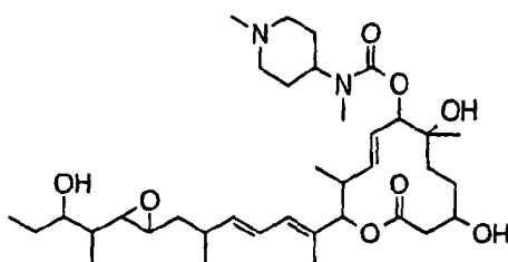
Compound B80
