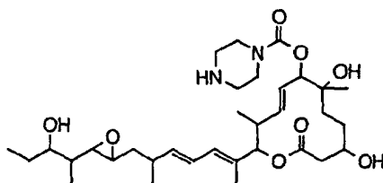
Compound B52
