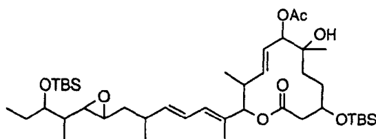
Compound B10-1
