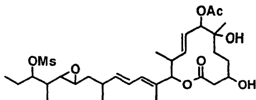
Compound B16-1
