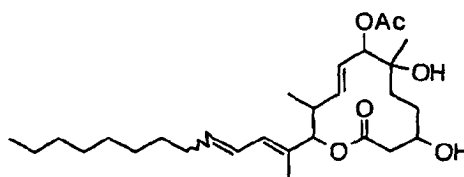
Compound 76
