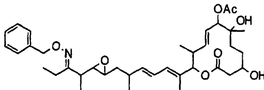
Compound B75
