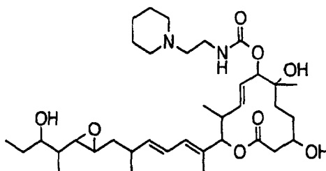
Compound B63
