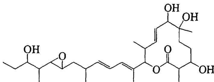
11107AI
