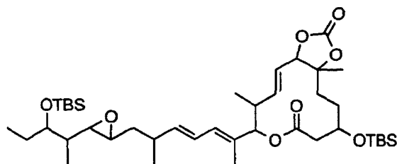
Compound B13
