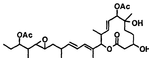
Compound B20-2
