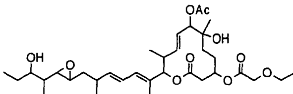
Compound B24
