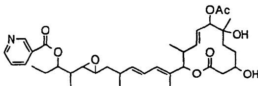
Compound B29
