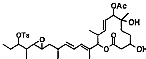
Compound B17
