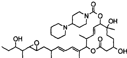
Compound B77
