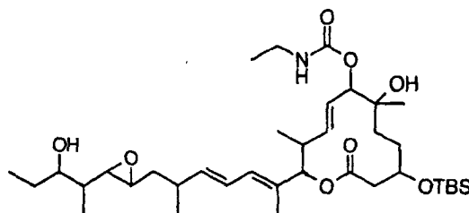
Compound B70
