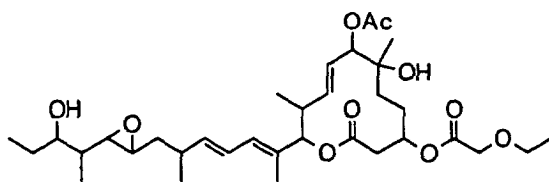
Compound B24
