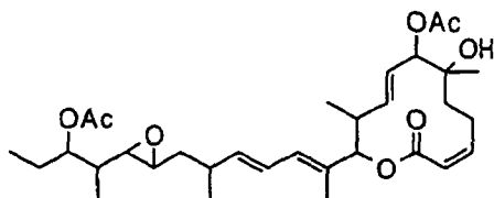
Compound B43-1
