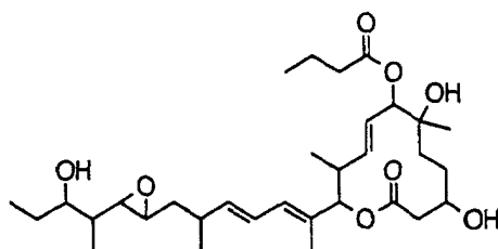
Compound 42
