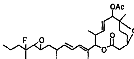
Compound B19-2
