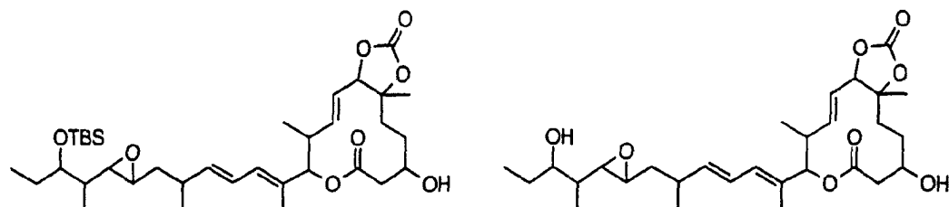
Compound B14-1
