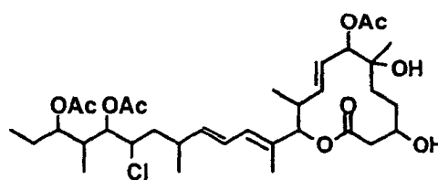
Compound B21-4
