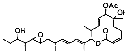
Compound B43-2
