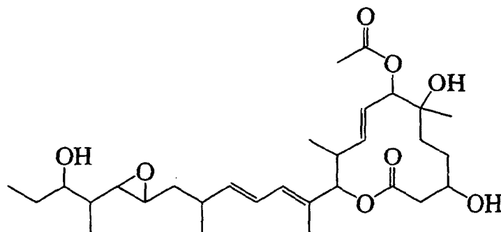
11107AD
