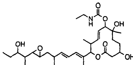
Compound B68
