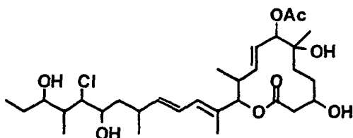
Compound B1-1
