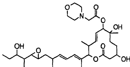
Compound B40
