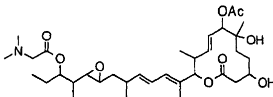
Compound B28
