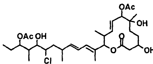
Compound B21-2
