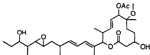
Compound B8-5
