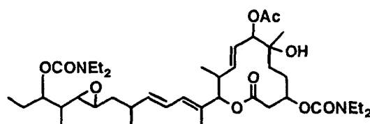
Compound B38
