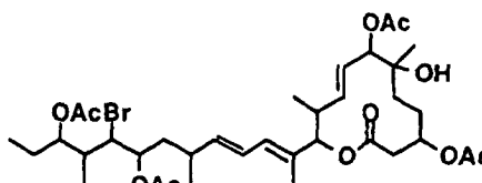
Compound B23-2
