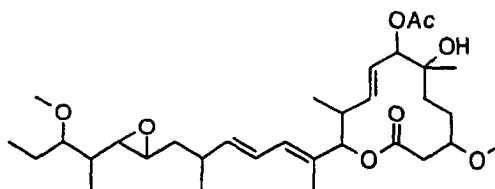
Compound B8-6
