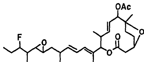
Compound B19-1
