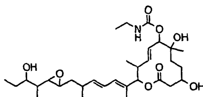
Compound B68
