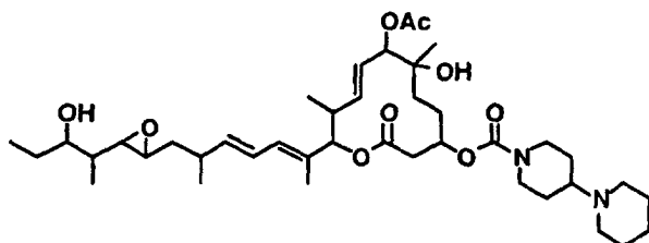
Compound B37-1
