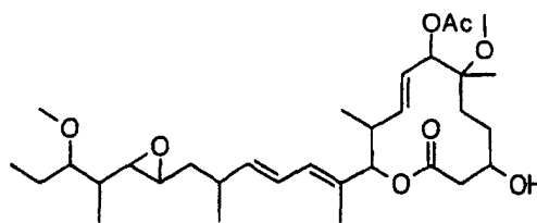
Compound B8-2
