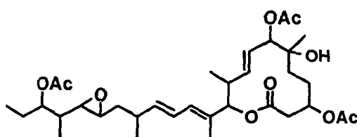
Compound B20-1
