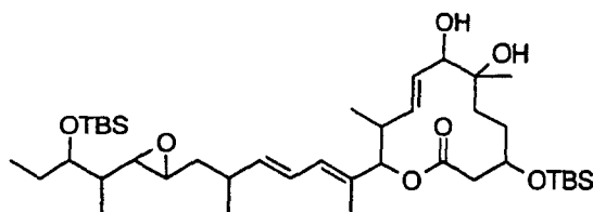
Compound B12
