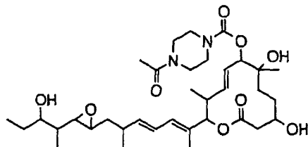
Compound B51
