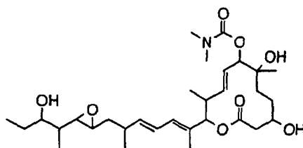
Compound B46
