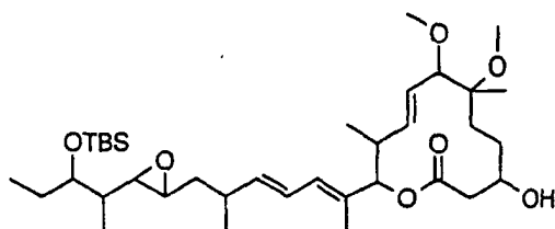
Compound B15-1
