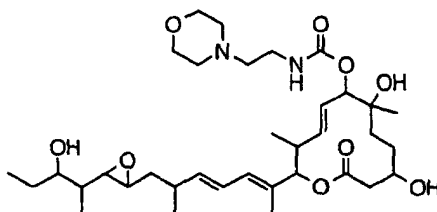
Compound B59
