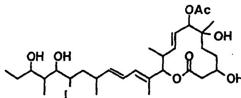
Compound B3-2
