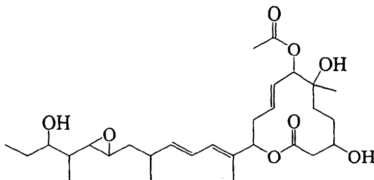
11107Z
