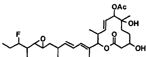
Compound B18-1
