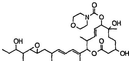
Compound B49
