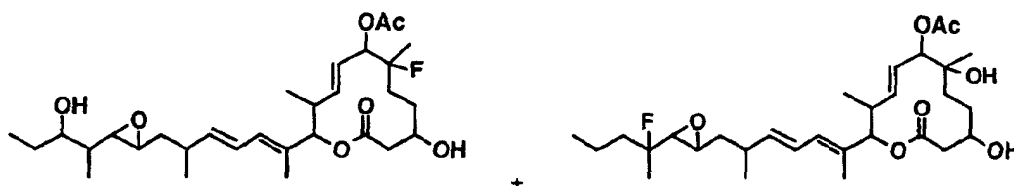
Compound B18-3
