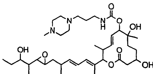
Compound B78
