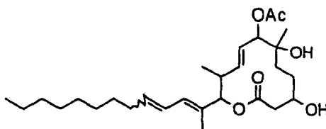
Compound B76
