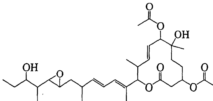
11107M
