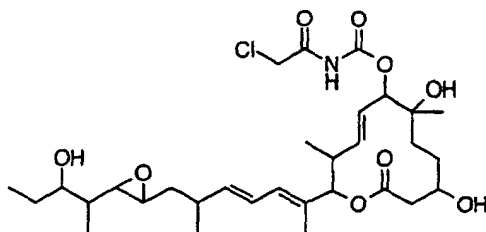
Compound B69
