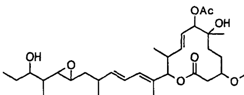
Compound B8-4
