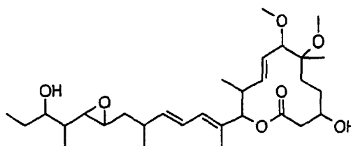
Compound B15-2
