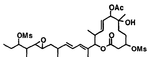
Compound B16-2
