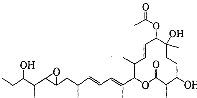
11107X
