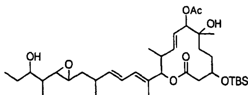
Compound B10-2
