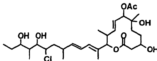
Compound B1-2
