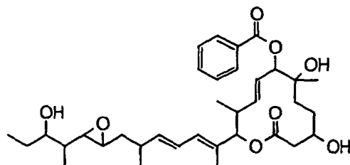
Compound B41
