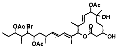
Compound B23-1
