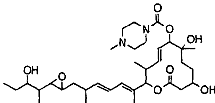
Compound B50
