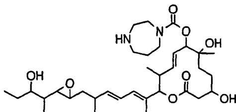
Compound B61
