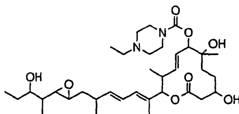
Compound B65
