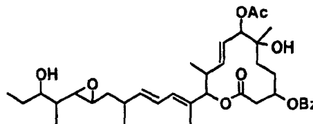
Compound B30-2
