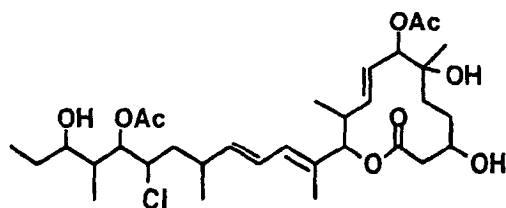
Compound B21-1
