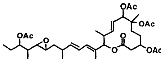
Compound B20-3
