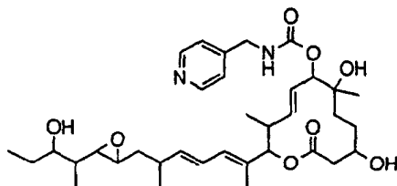
Compound B58
