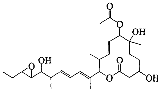
11107AY
