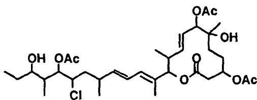
Compound B21-3
