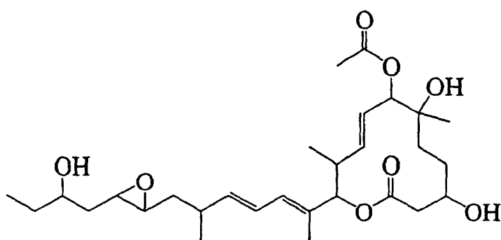
11107T
