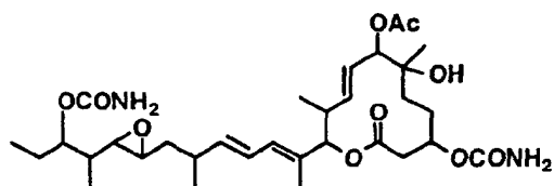
Compound B33-1
