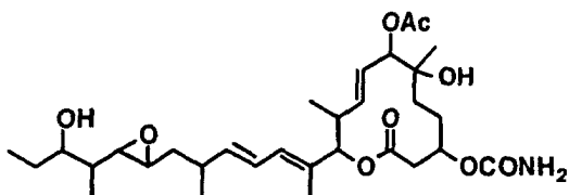
Compound B35-1
