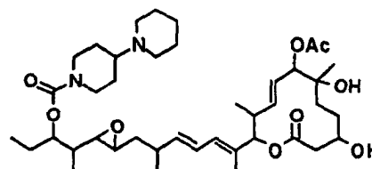
Compound B37-2
