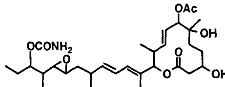
Compound B35-2
