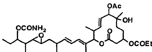
Compound B33-2
