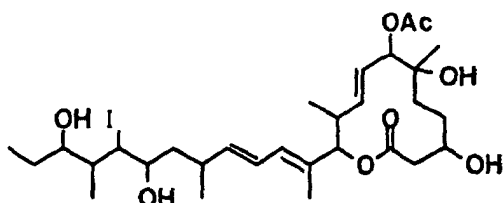
Compound B3-1
