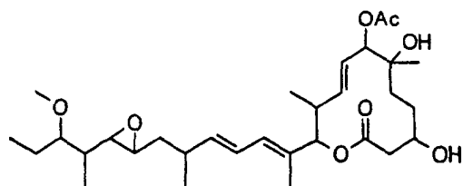
Compound B8-1
