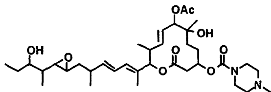
Compound B36-1
