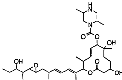
Compound B67
