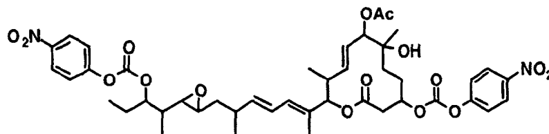
Compound B32
