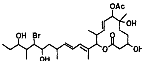
Compound B2-2
