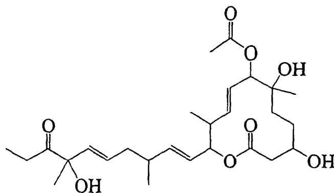
11107AH
