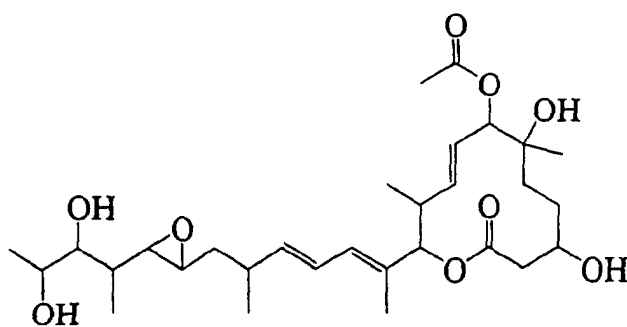
11107AW
