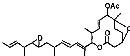
Compound B19-3
