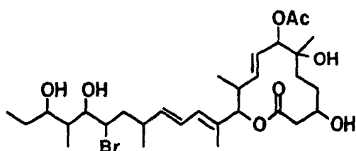
Compound B2-1
