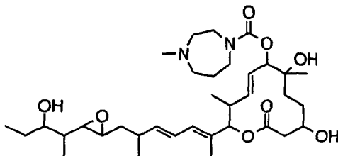
Compound B62
