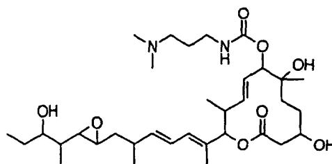
Compound B55
