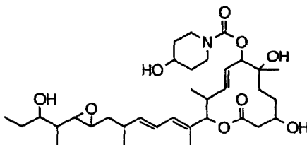
Compound B48
