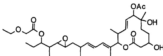
Compound B25
