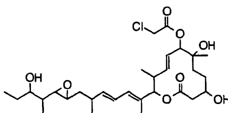
Compound B39
