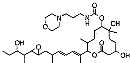
Compound B60
