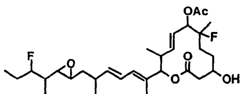
Compound B18-4
