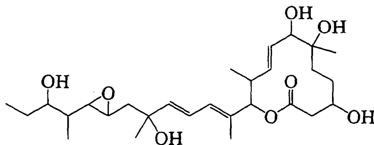
11107F
