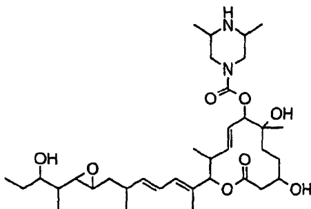
Compound B81
