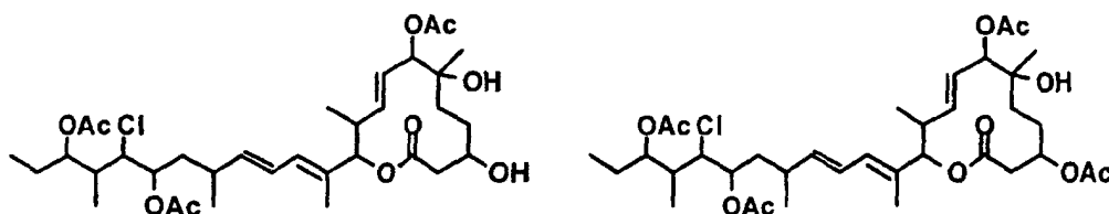
Compound B22-1
