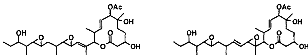
Compound B31
