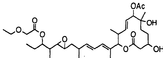
Compound B25
