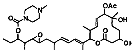
Compound B36-2
