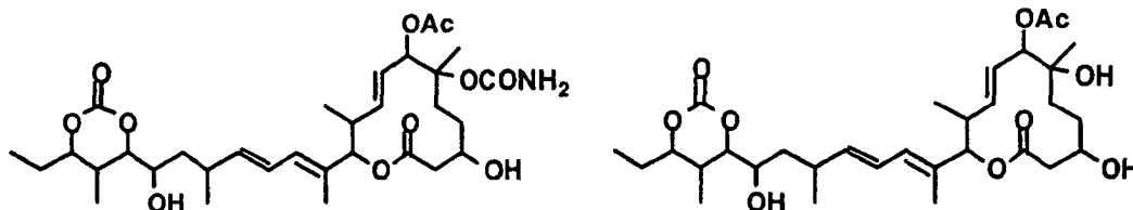
Compound B34-1
