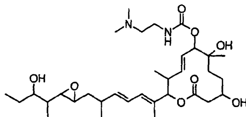
Compound B54
