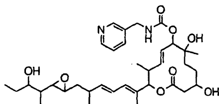
Compound B57
