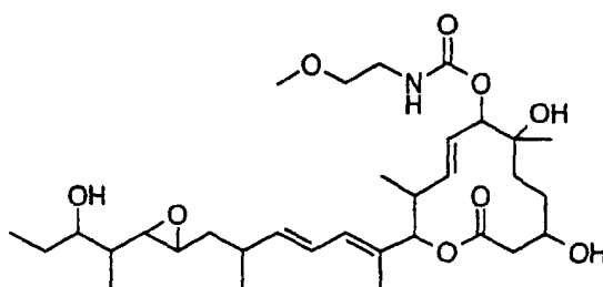
Compound B53
