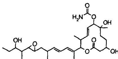
Compound B44
