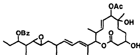
Compound B30-3
