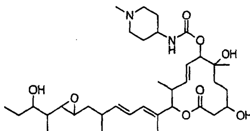
Compound B77
