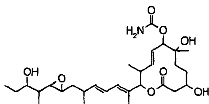
Compound B44
