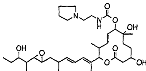
Compound B64
