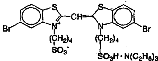
Spectral sensitizing dye 2
