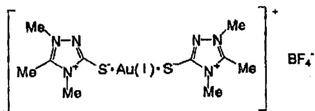
Gold sensitizing agent 1
