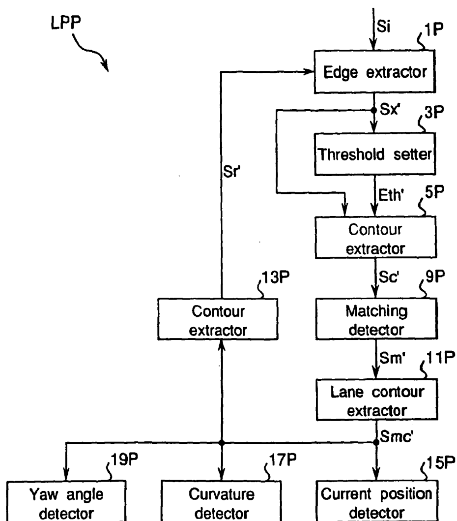
Fig.25 PRIOR ART
