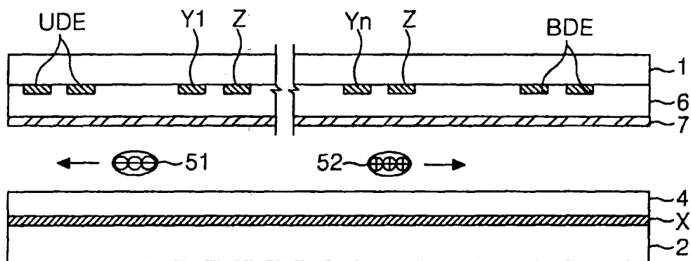
FIG. 5 RELATED ART
