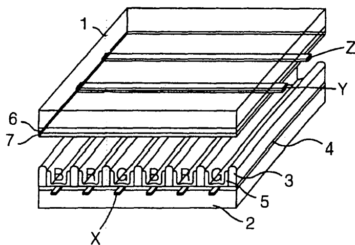
FIG.1 RELATED ART
