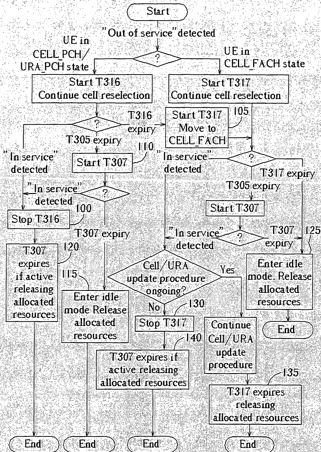
Fig. 4 Prior art
