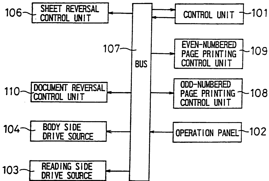
FIG. 17 PRIOR ART
