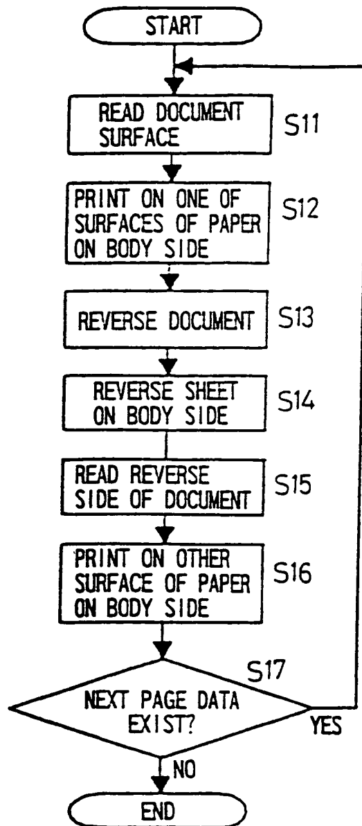
FIG. 18 PRIOR ART
