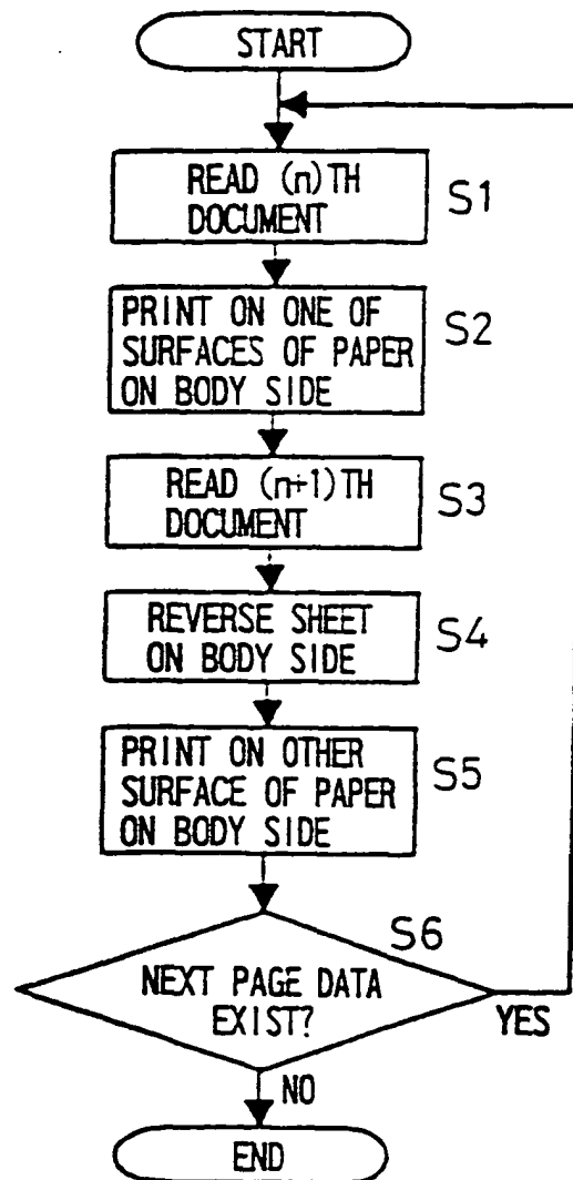
FIG. 16 PRIOR ART
