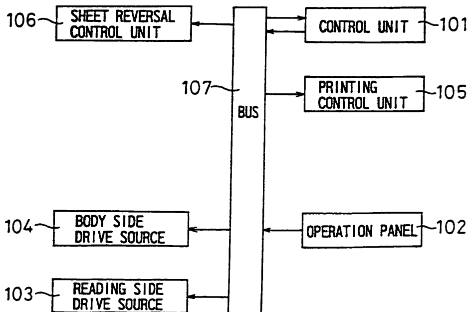
FIG. 15 PRIOR ART
