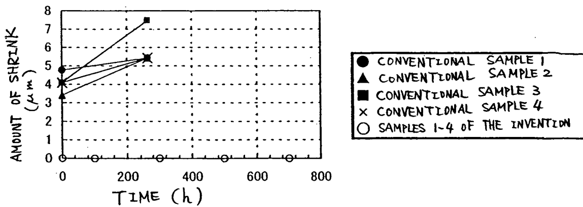
Fig. 4 CHANGE OF AMOUNT OF SHRINK WITH TIME PASSING UNDER 65°C AND % RH
