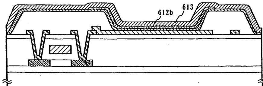
Fig.6D FORMATION OF SECOND LAYER CONTAINING ORGANIC COMPOUND, AND CATHODE (VAPOR DEPOSITION METHOD)
