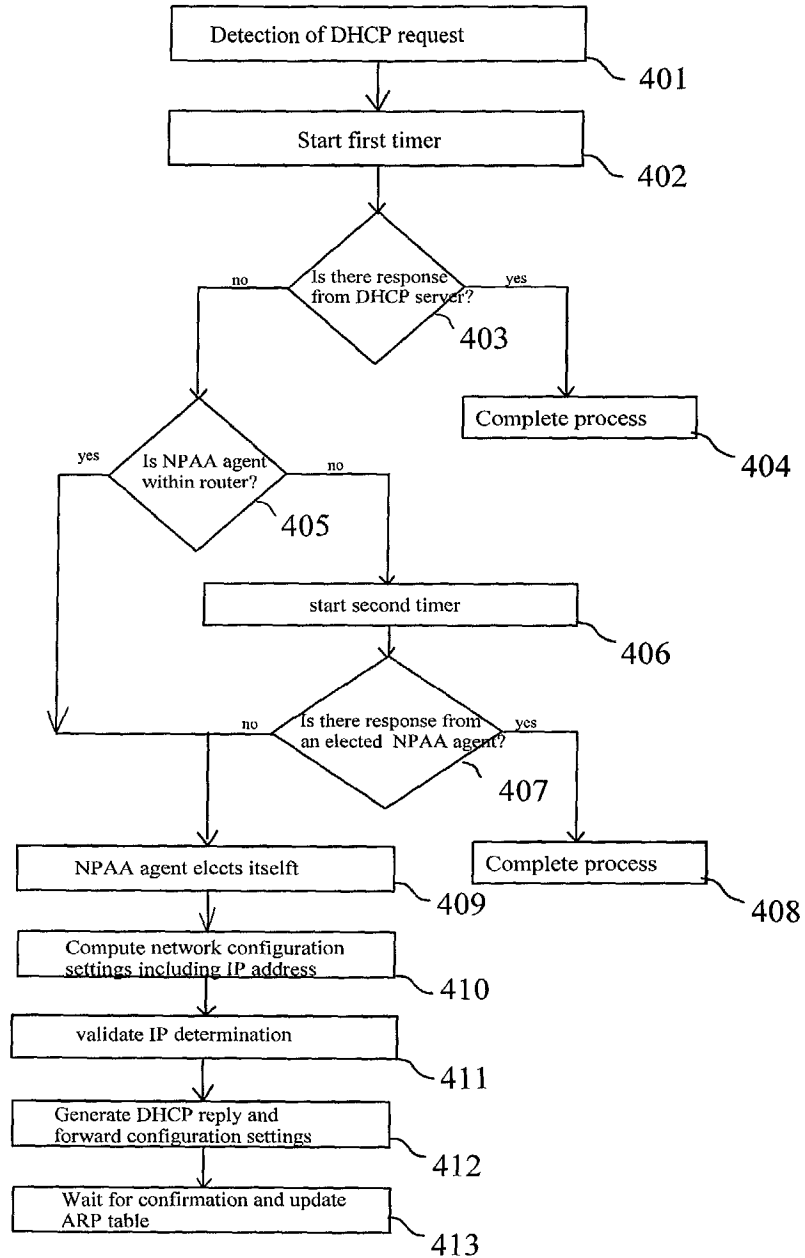
Fig. 4: NPAA election process
