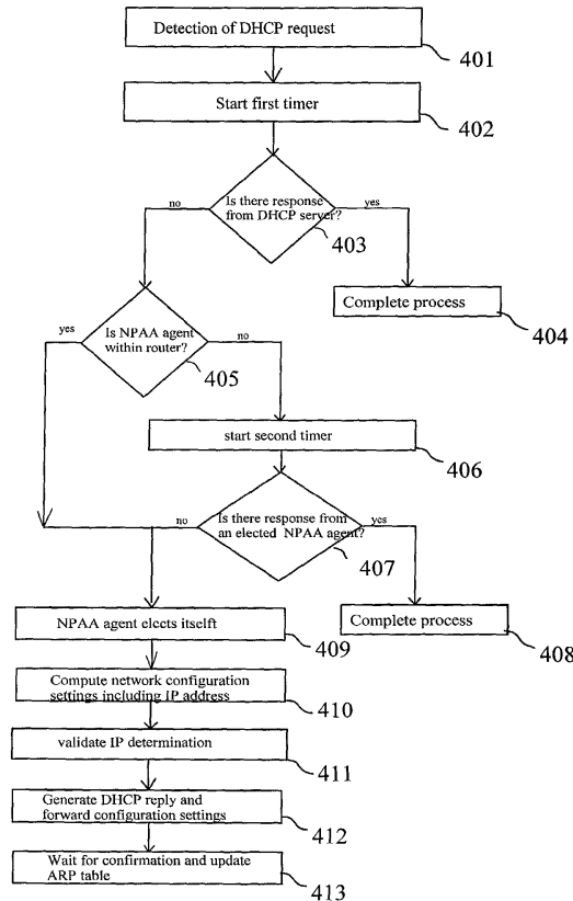
Fig. 4: NPAA election process
