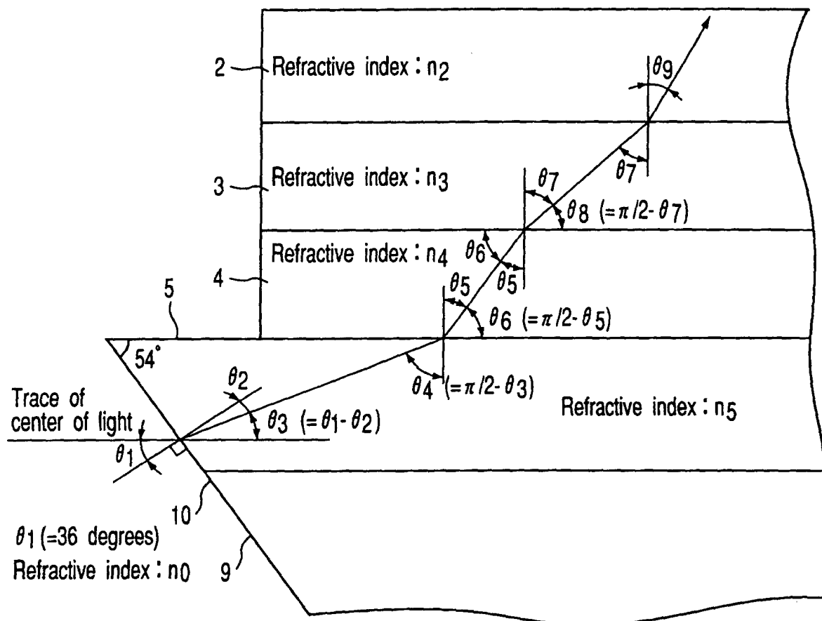
FIG. 16 (PRIOR ART)
