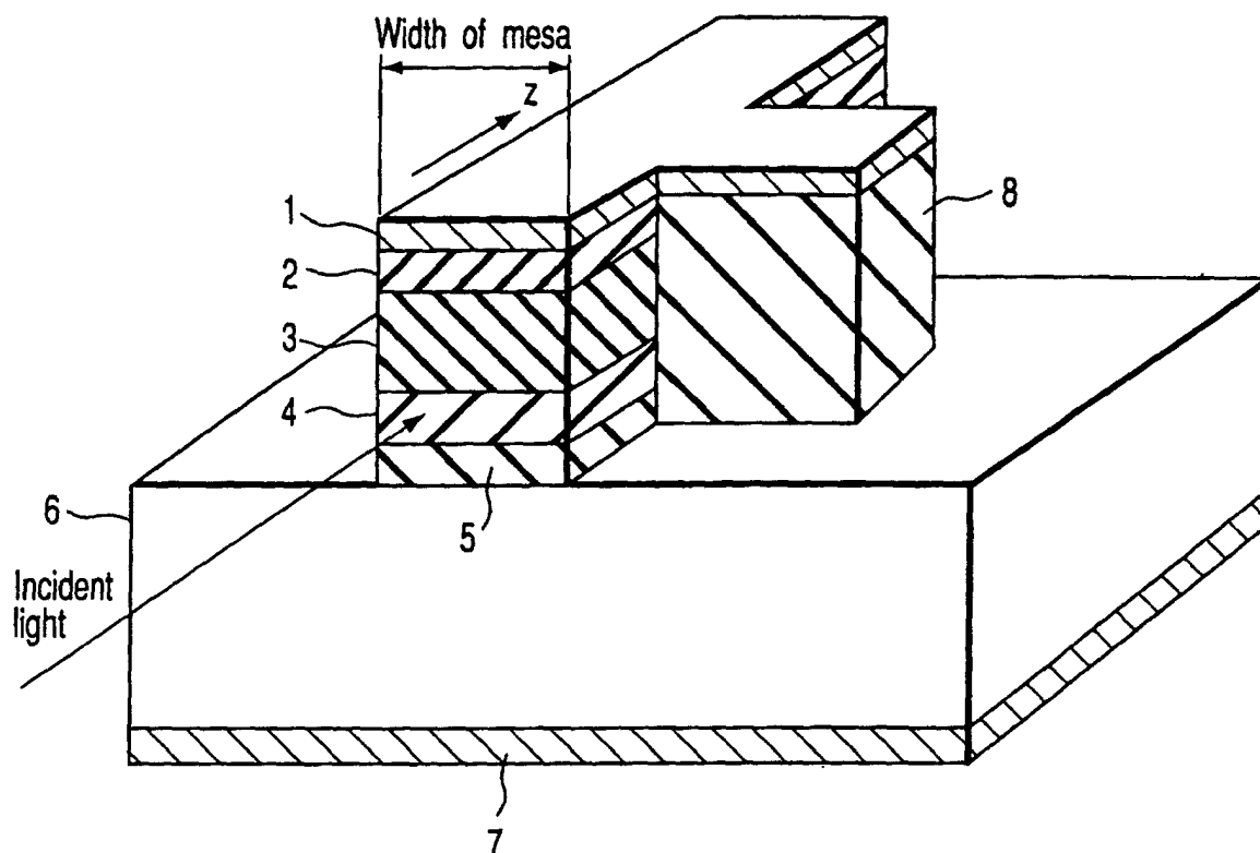
FIG. 12 (PRIOR ART)
