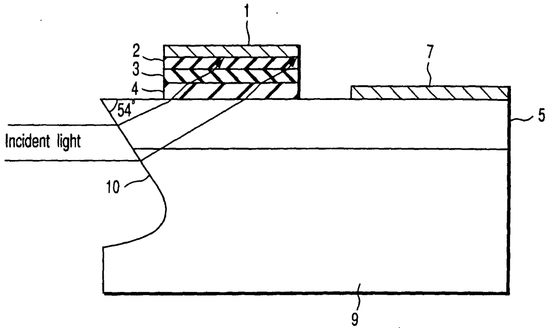
FIG. 14 (PRIOR ART)
