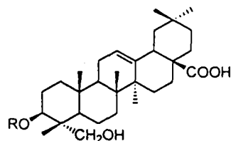
Hederagenin ; R = H Hederagenin 3-O- \beta -D-glucopyranoside ; R = glc Patensin ; R = glc-gal
