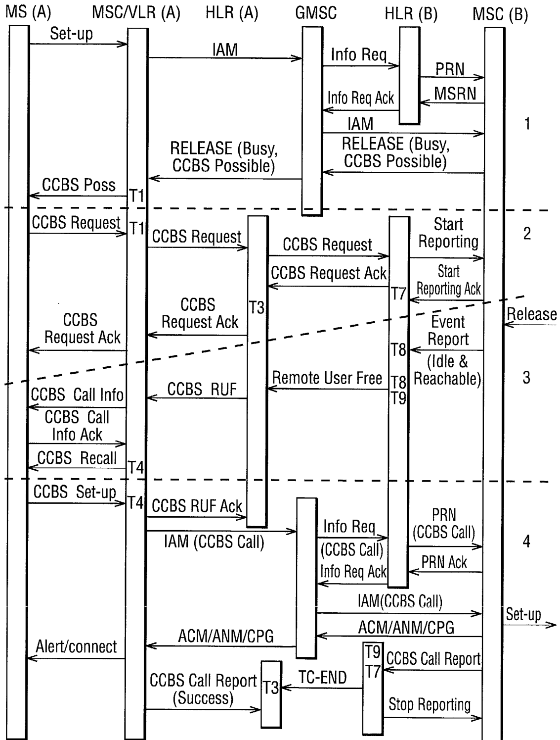
FIG. 1 (Prior Art) CCBS Functionality
