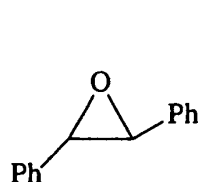
Racemic form (a)
