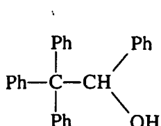
Racemic form (b)
