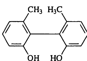
Racemic form (c)
