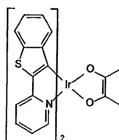
Btp 2 (acac)
