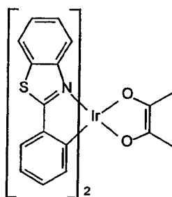
Bt 2 (acac)
