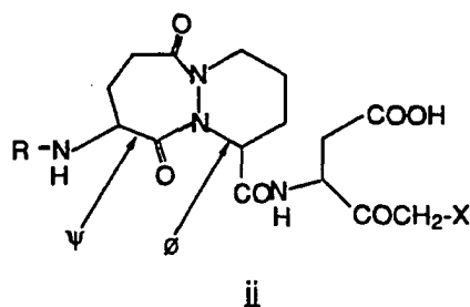
[7,6]-Bicyclic lactam-based ICE inhibitor (the invention)
