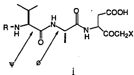
Peptide-based ICE inhibitor (Dolle, R.E. et al., J. Med. Chem (1994) 37 , 563)
