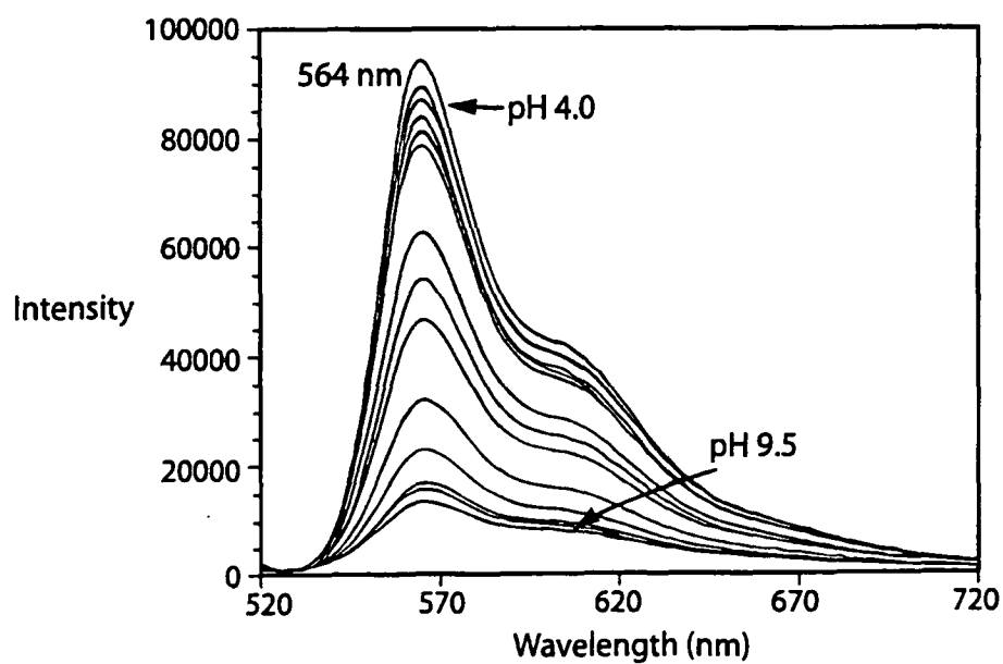
Fig. 2 CY3.39 acid ex at 514 nm in pH 4.0-9.5
