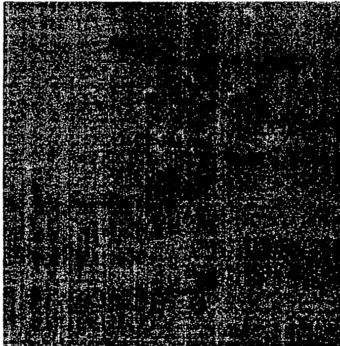
Fig. 8 The internalization of pH sensitive Cy5
