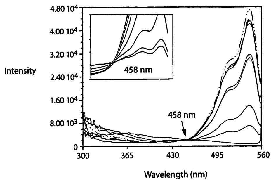
Fig. 3 excitation spectrum of CY 3H pH/564 nm emit
