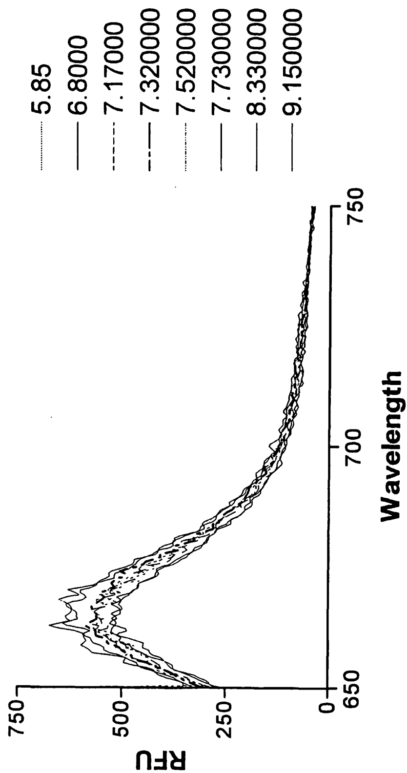
Fig. 7 pH Sensitive Tandem Dye Energy Transfer Cassette (Compound 11) (Excitation 630nm)
