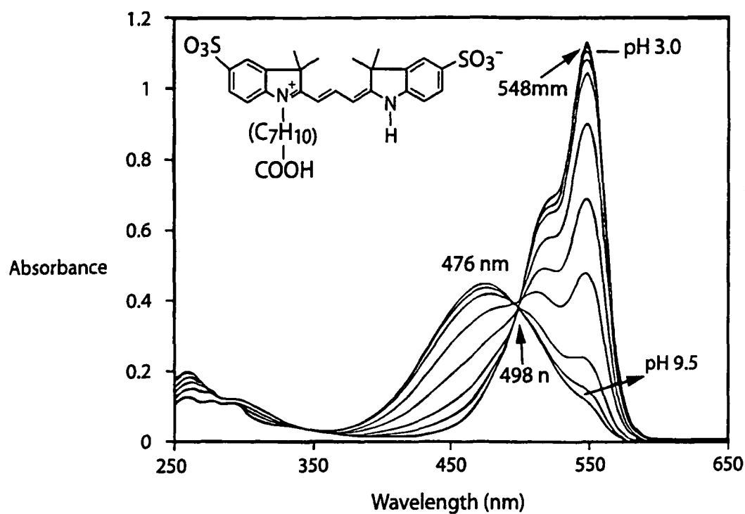
Fig. 1 CY3.39 acid absorption spectra in pH 3-9.5
