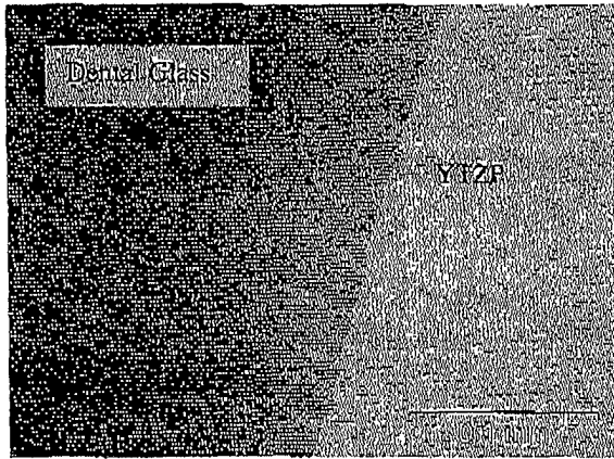
Figure 6. Dental Glass pressed to YTZP zirconia without the use of a liner
