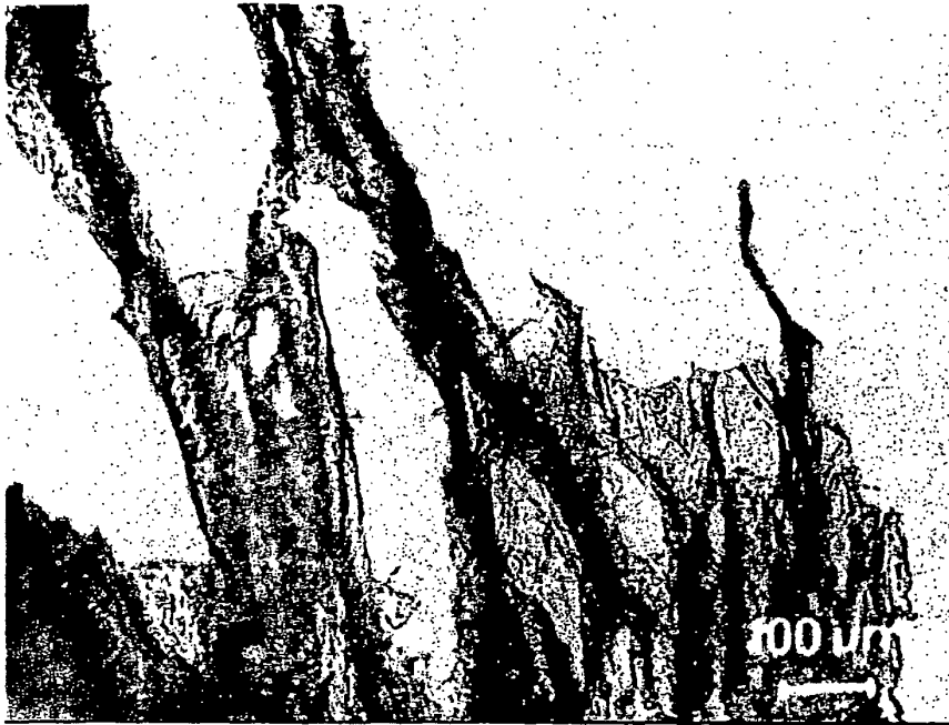
VERTICAL CROSS SECTION, x80 OPTICAL MICROSCOPE (TRANSMITTED LIGHT)
