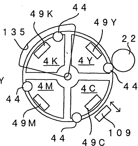
FIG. 37 B: DEVELOPING POSITION
