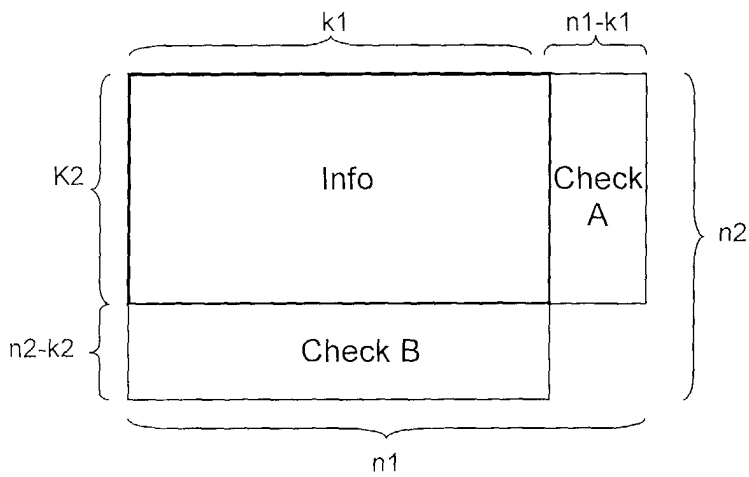
Fig. 2a (prior-art)
