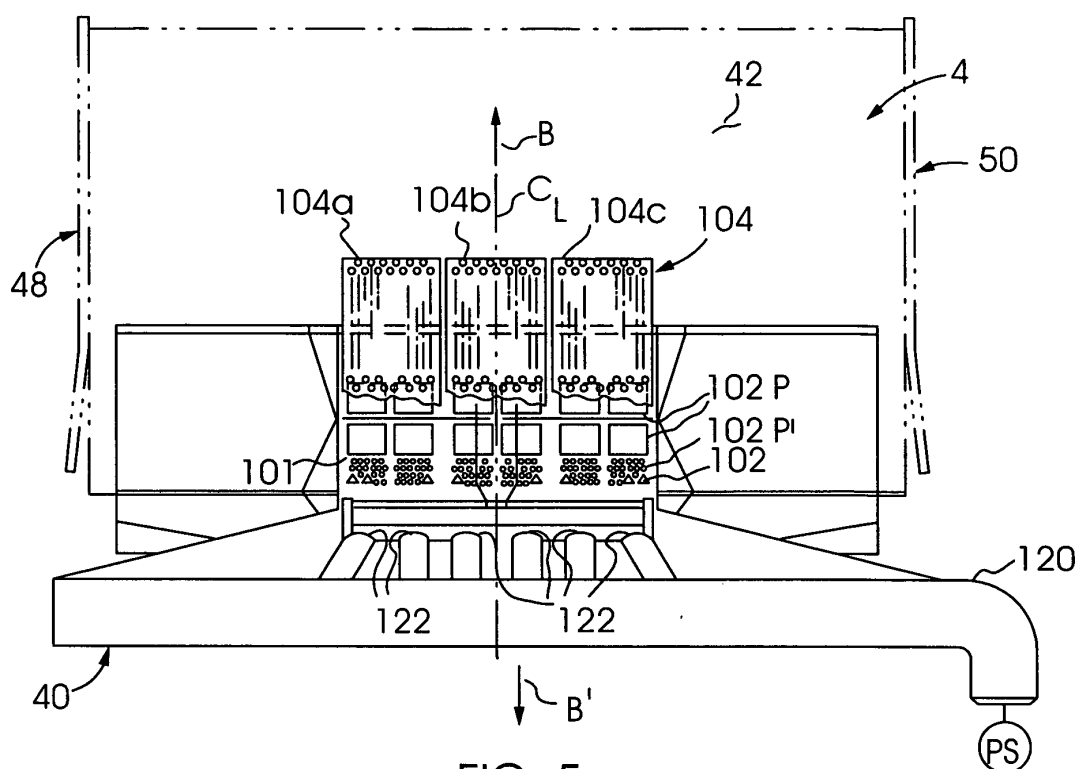
FIG. 5 (PRIOR ART)
