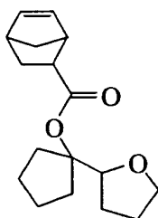
(Monomer 6)
