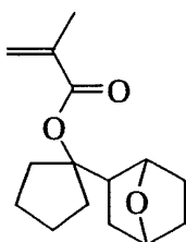
(Monomer 5)
