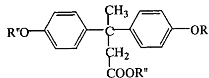
(AI-3)
