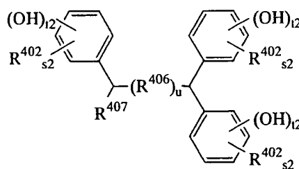
(A5)
