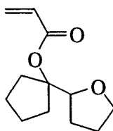
(Monomer 1)
