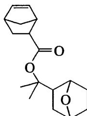
(Monomer 7)
