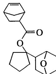
(Monomer 8)
