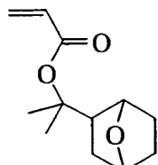
(Monomer 2)
