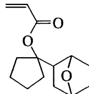
(Monomer 4)
