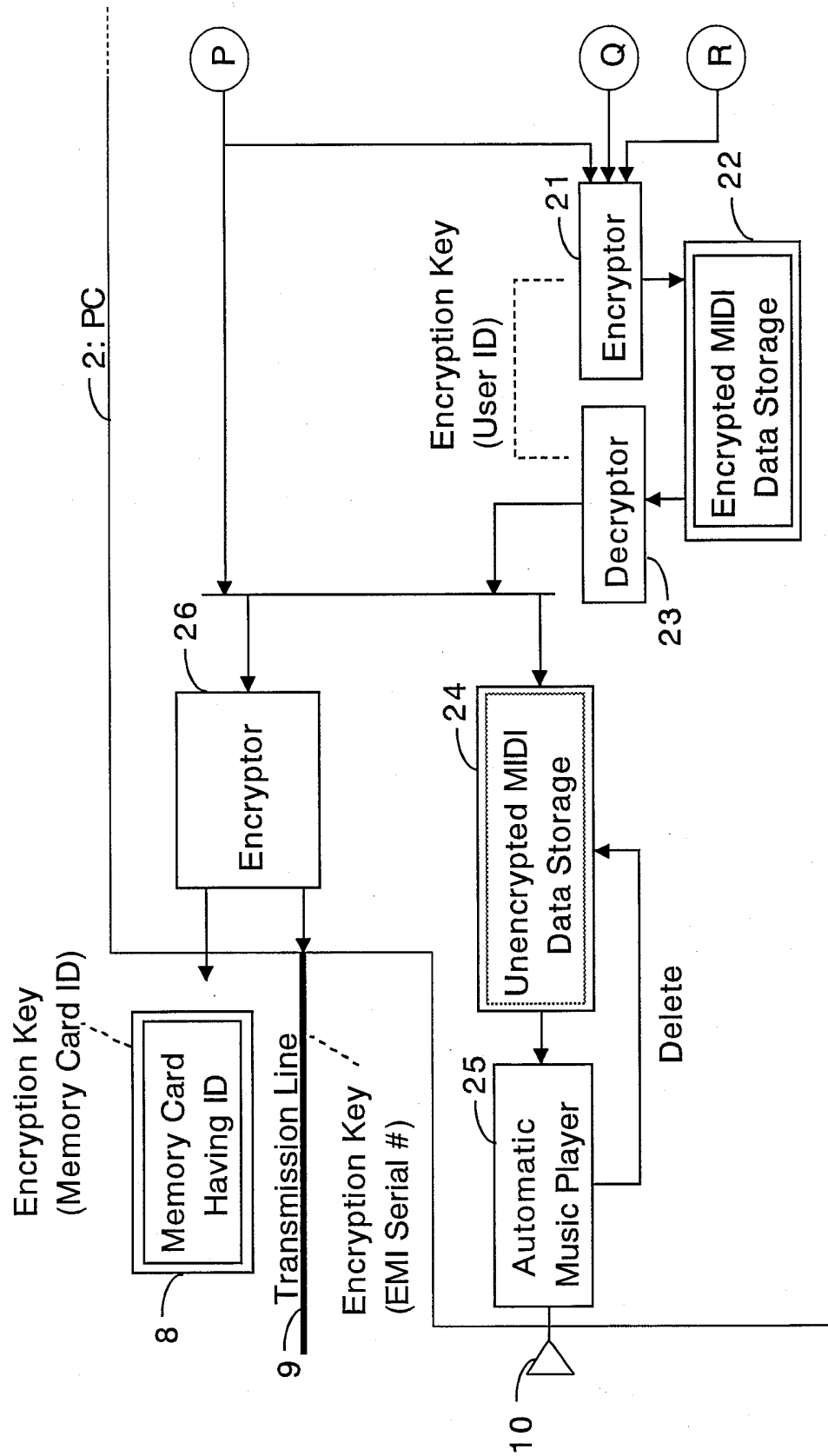
Fig. 1b System Configuration (Part 2)
