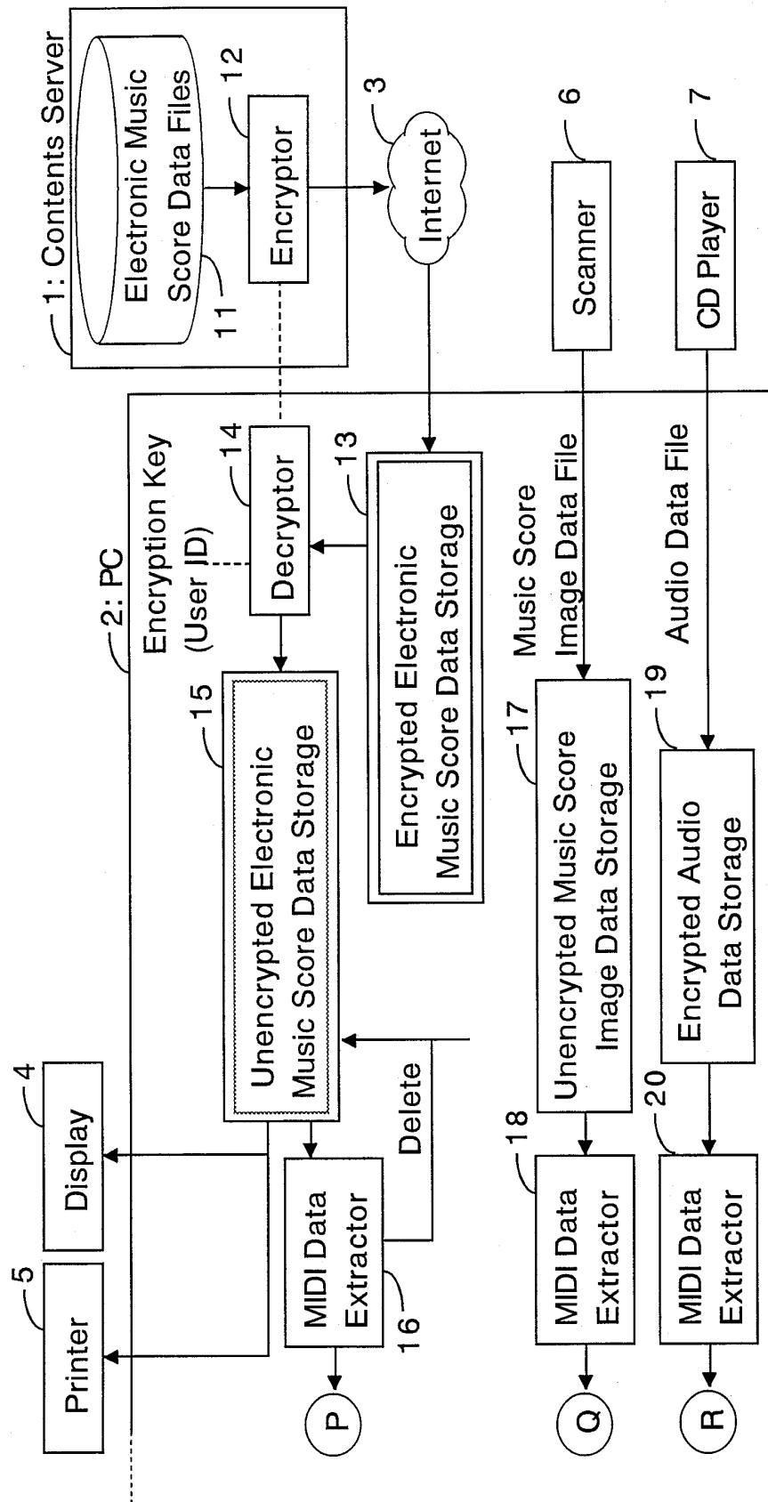
Fig. 1a System Configuration (Part 1)
