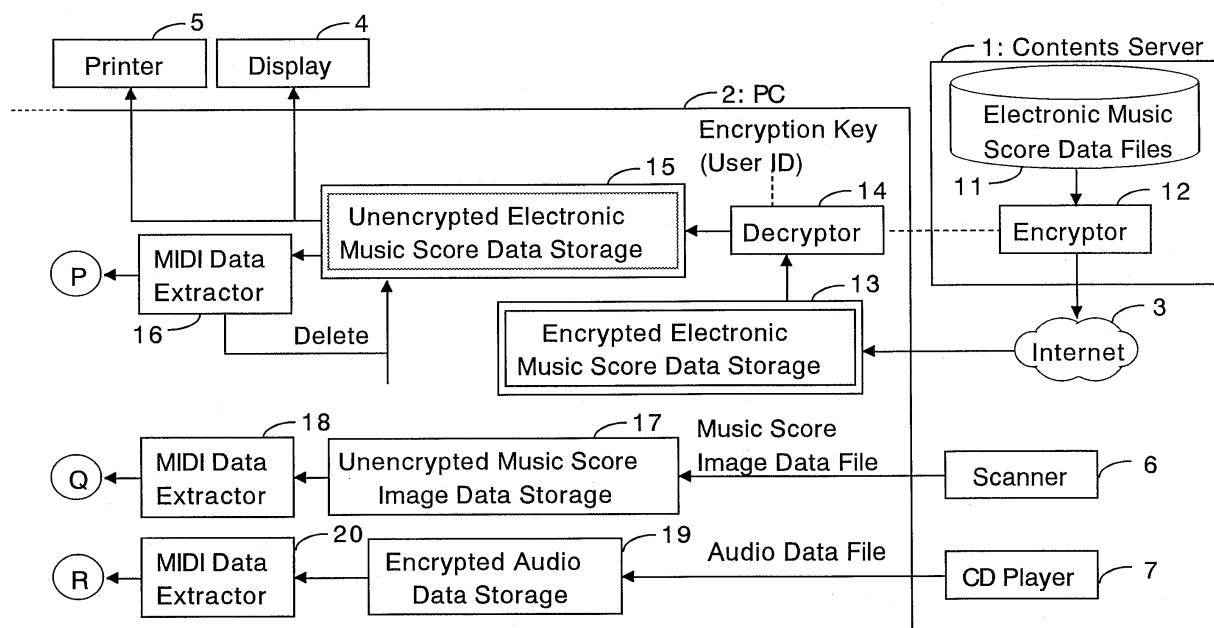
Fig. 1a System Configuration (Part 1)
