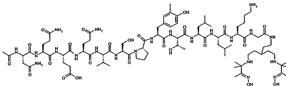
Figure 2: Chemical Structure of Compound 5 – The Peptide-chelator Conjugate Ac-Asn-Gln-Glu-Gln-Val-Ser-Pro-(I-Tyr)-Thr-Leu-Leu-Lys-Gly-[Compound 1].
