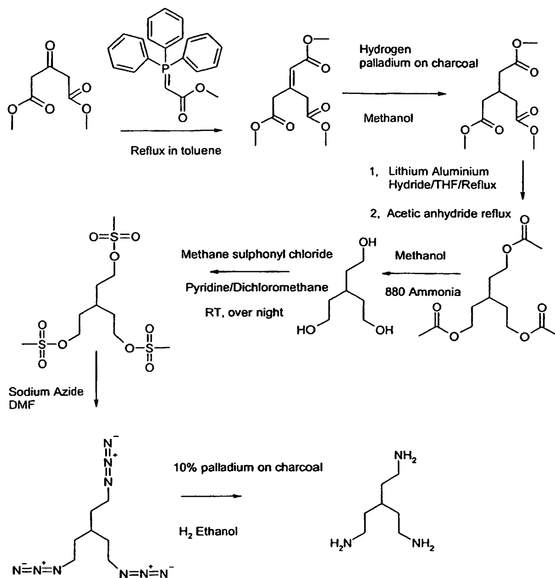
Figure 3: Azide Route to 1,1,1- tris (2-aminoethyl)methane.
