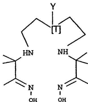
Figure 1: Chemical Structures of Compounds 1 to 6.
