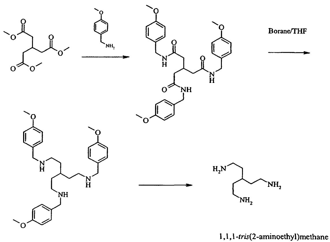
Figure 4: Alternative Synthesis of 1,1,1- tris (2-aminoethyl)methane.
