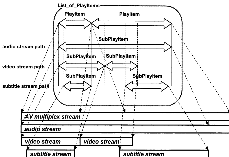
Figure 1: List_of_PlayItems Example
