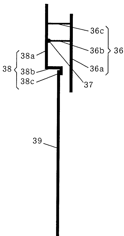
CROSS-SECTIONAL SIDE VIEW OF TWO-CONNECTED BASE PLATES
