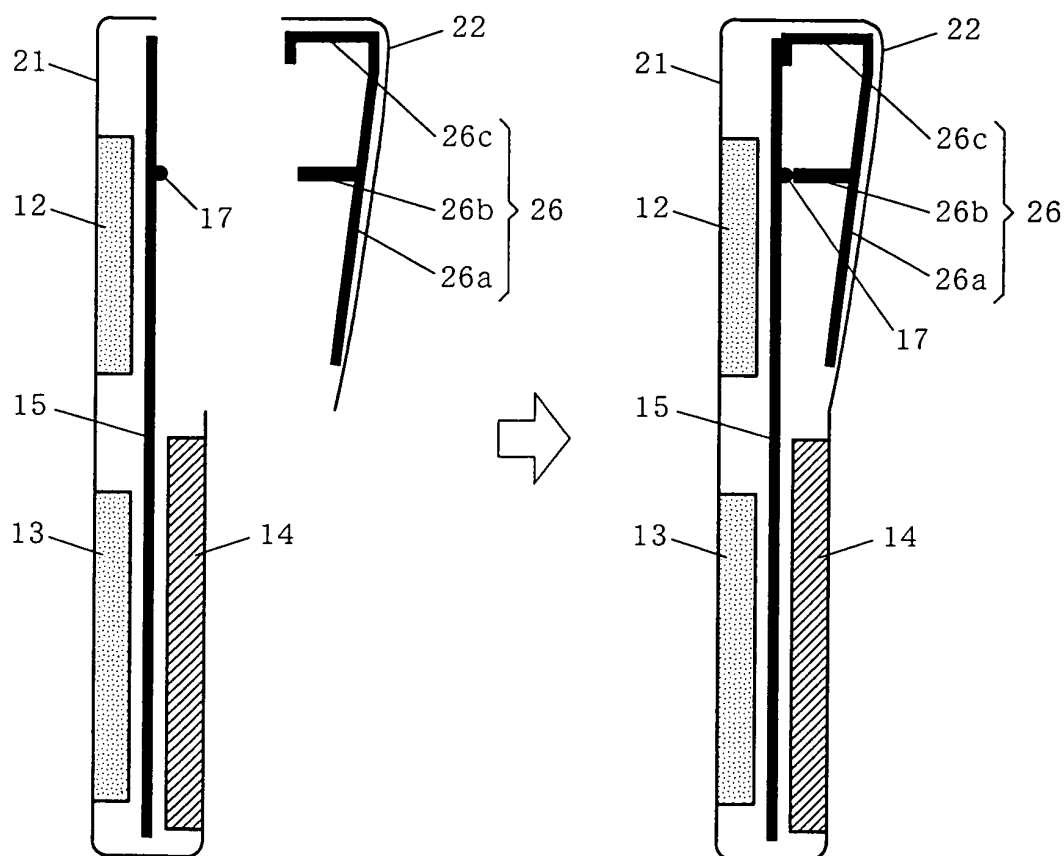
CROSS-SECTIONAL SIDE VIEW (TWO-PIECE)
