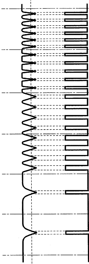
FIG. 4A OUTPUT SIGNAL FROM SIGNAL METER OUTPUTTING CIRCUIT
