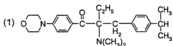
1-[4-morpholinophenyl]-2-dimethylamino-2-(4-isopropylbenzyl)-butane-1-one
