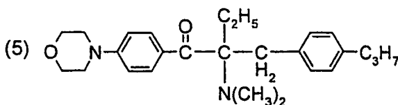
1-[4-morpholinophenyl]-2-dimethylamino-2-(4-n-propylbenzyl)-butane-1-one
