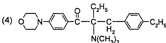
1-[4-morpholinophenyl]-2-dimethylamino-2-(4-ethylbenzyl)-butane-1-one
