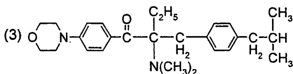
1-[4-morpholinophenyl]-2-dimethylamino-2-[4-(2-methylprop-1-yl)-benzyl]-butane-1-one
