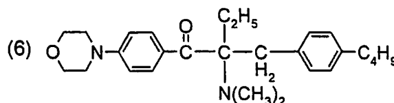
1-[4-morpholinophenyl]-2-dimethylamino-2-(4-n-butylbenzyl)-butane-1-one
