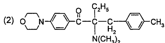
1-[4-morpholinophenyl]-2-dimethylamino-2-(4-methylbenzyl)-butane-1-one
