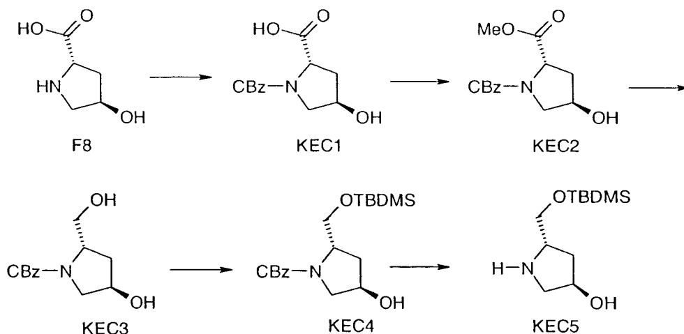
Scheme 6
