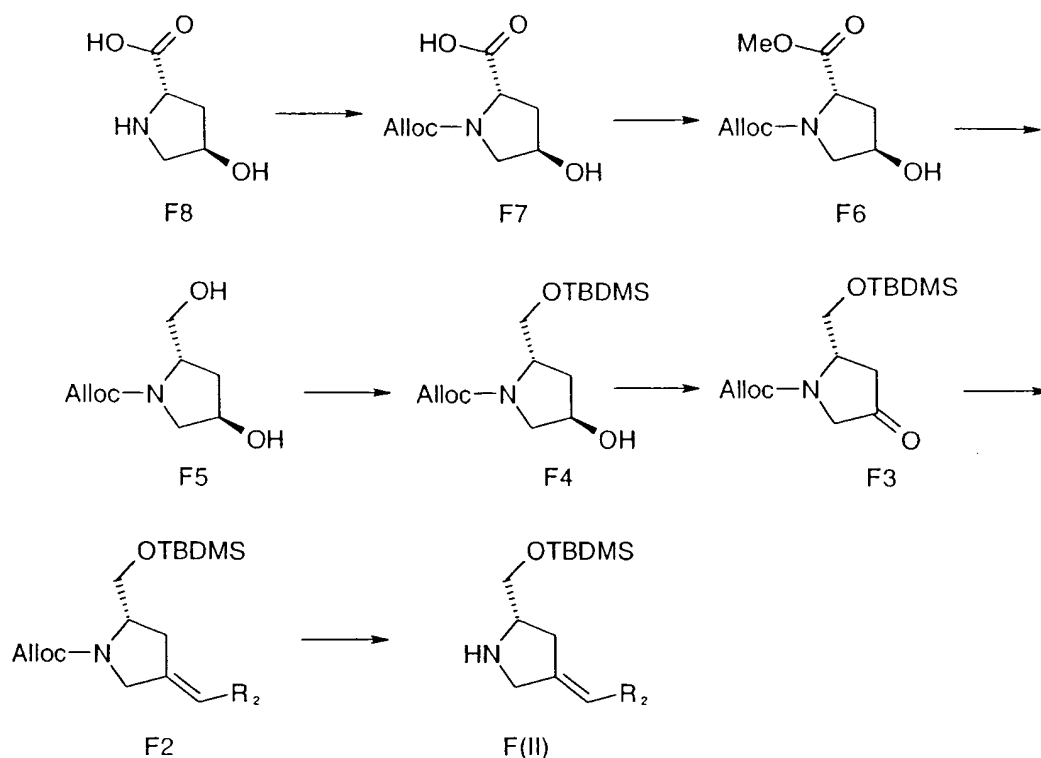
Scheme 8
