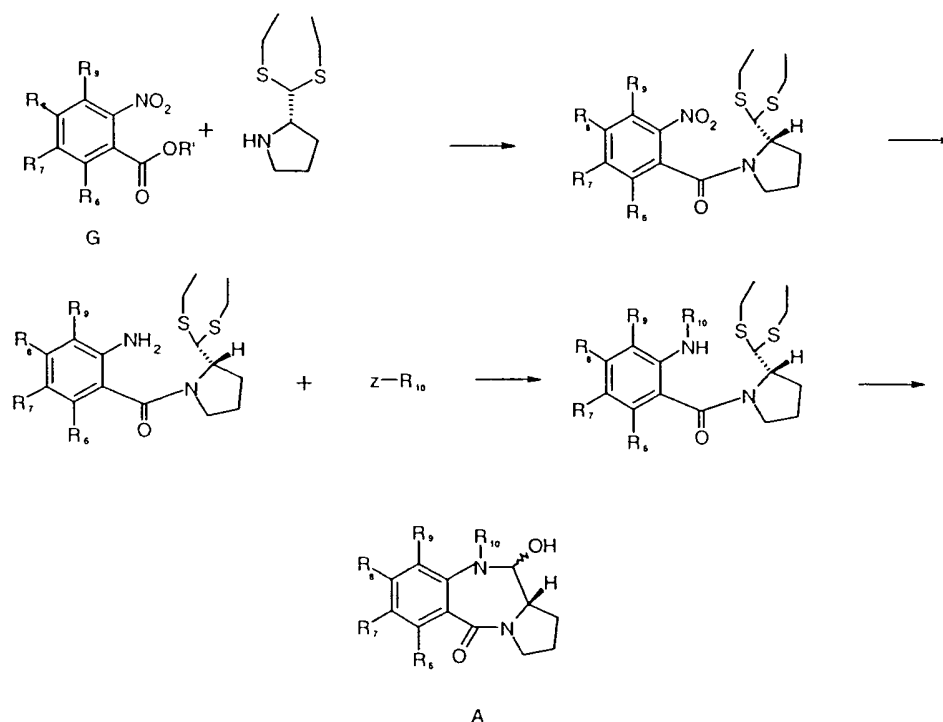
Scheme 2
