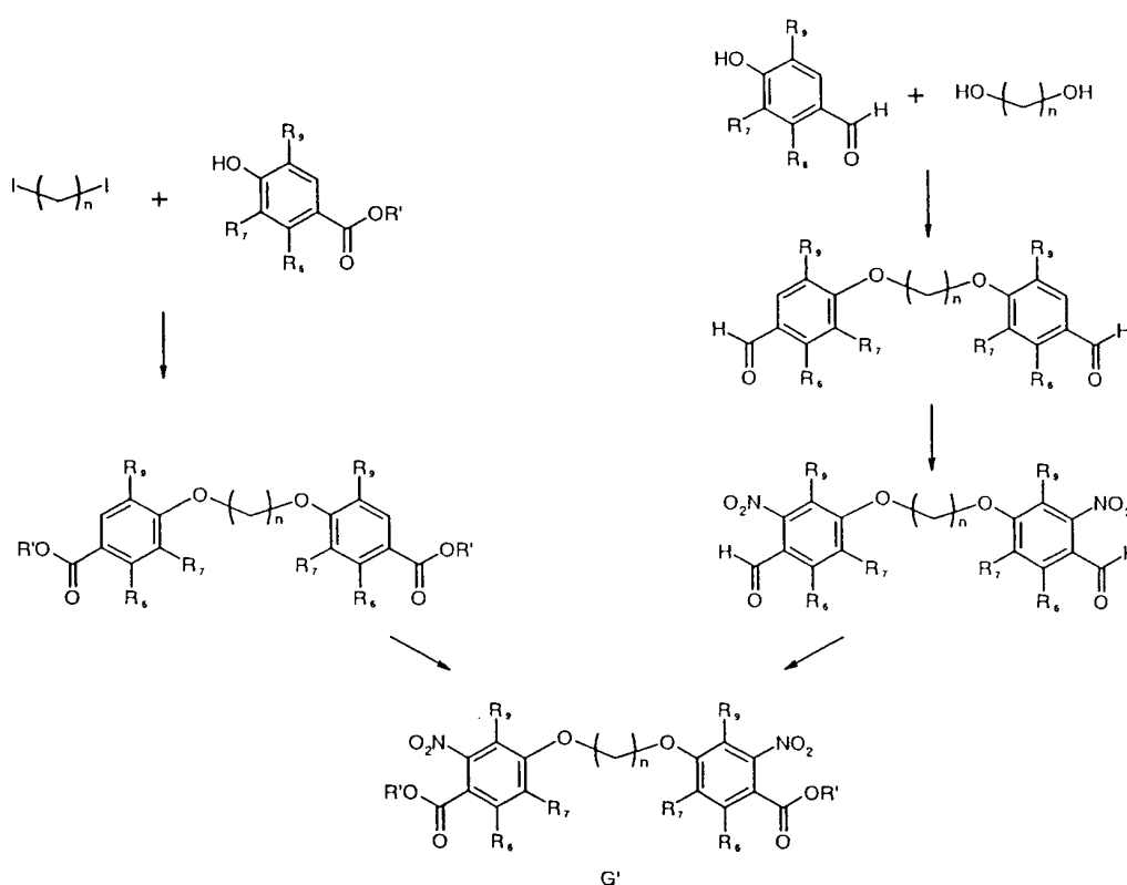
Scheme 3
