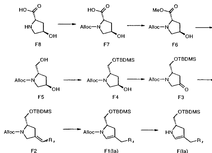
Scheme 4
