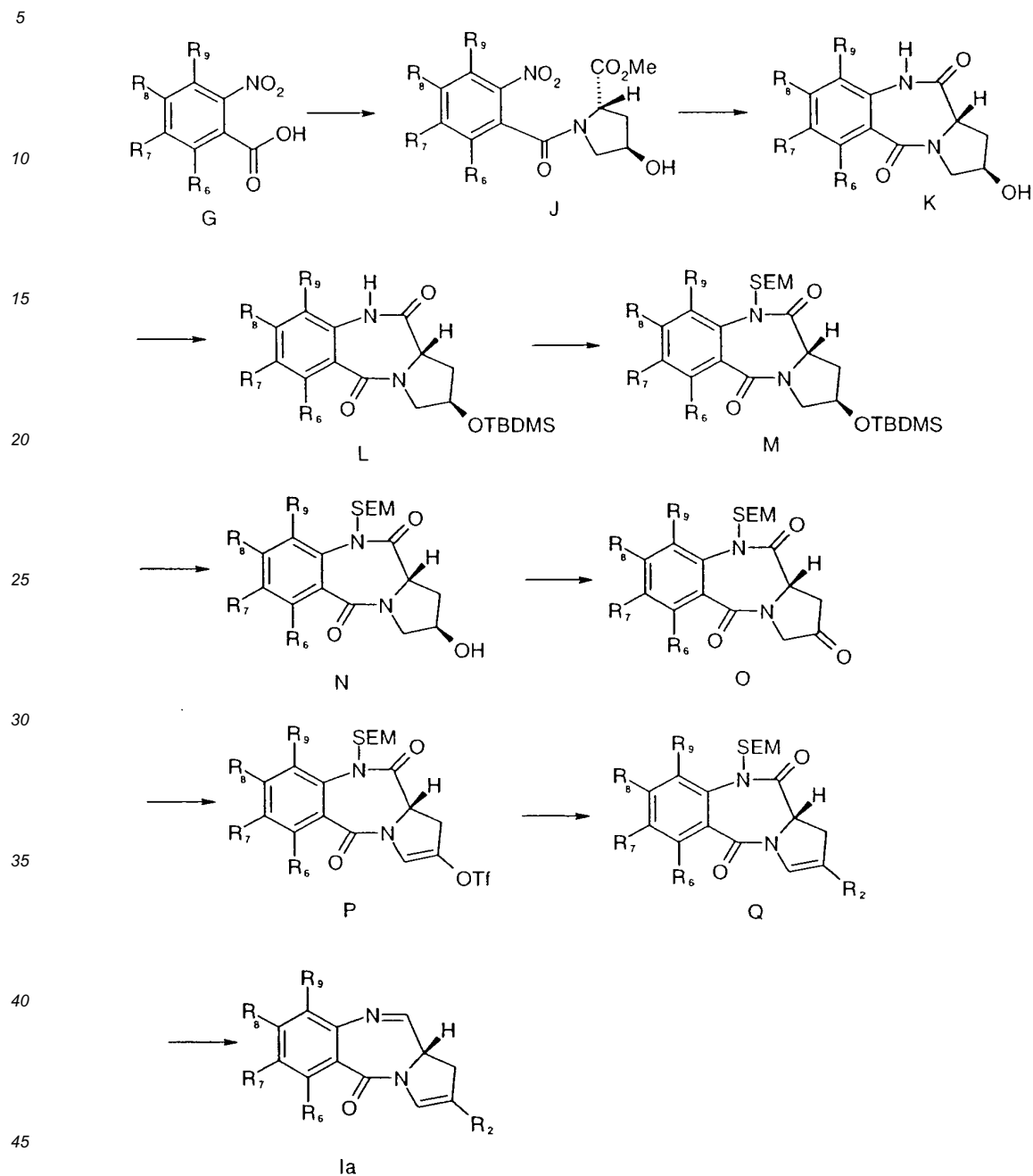
Scheme 7
