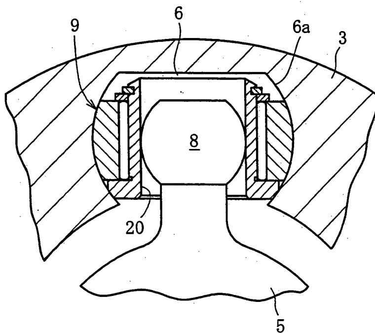
Fig. 19 PRIOR ART
