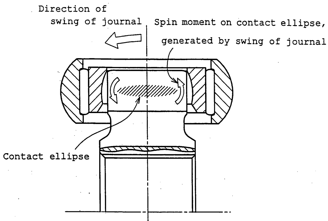
Fig. 18 PRIOR ART
