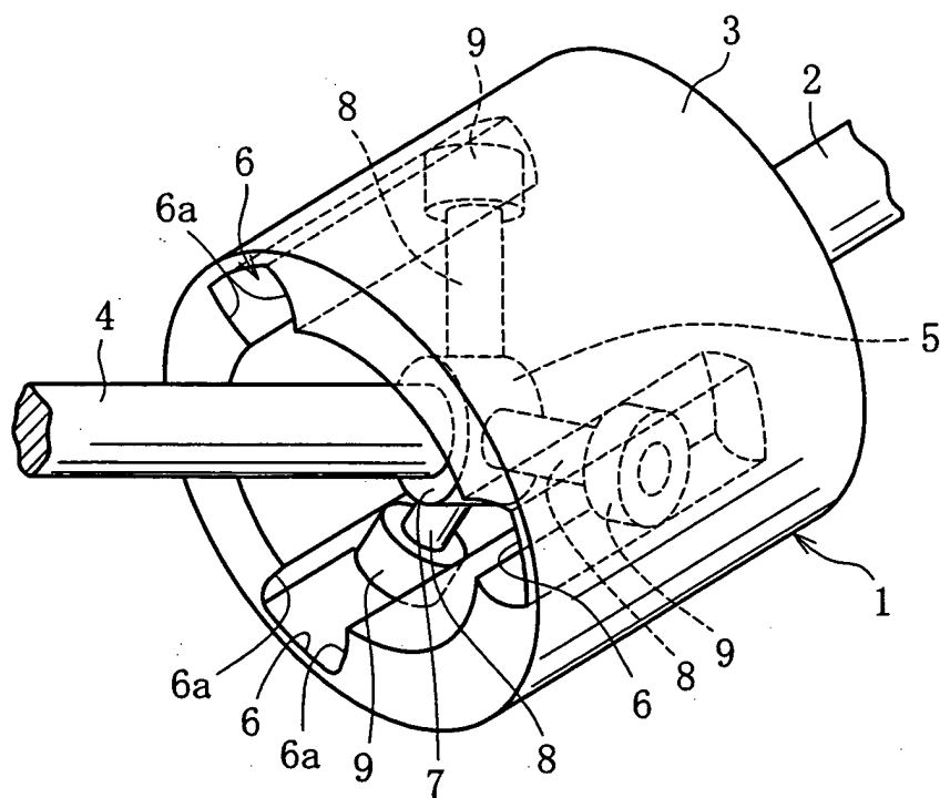
Fig. 16 PRIOR ART
