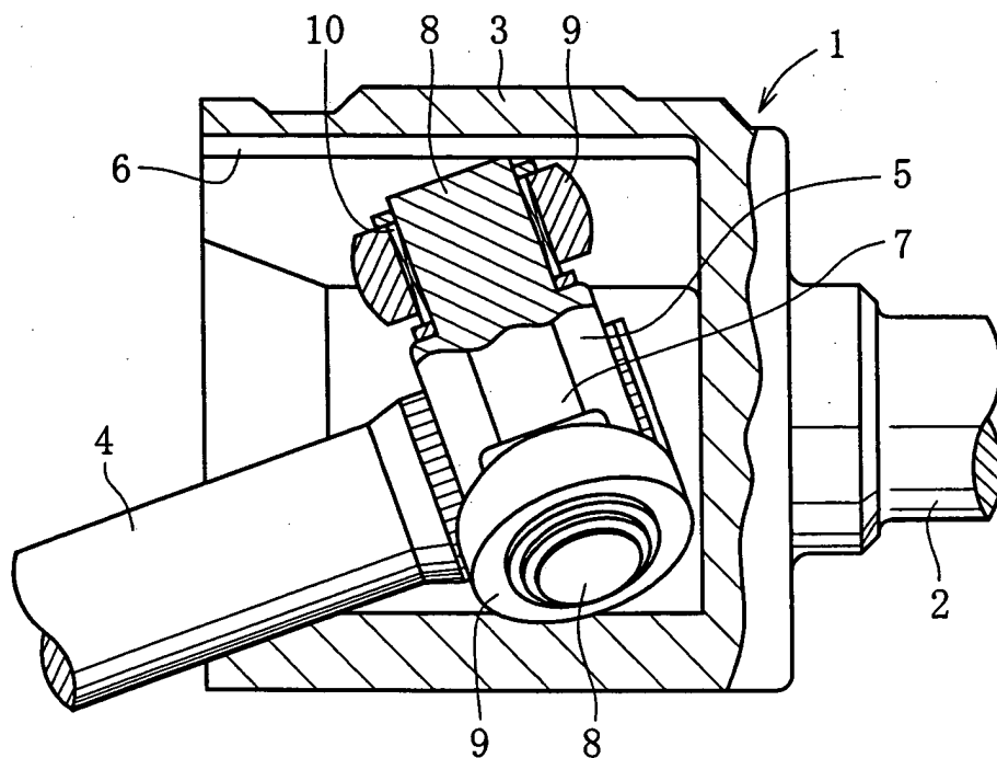
Fig. 16 PRIOR ART
